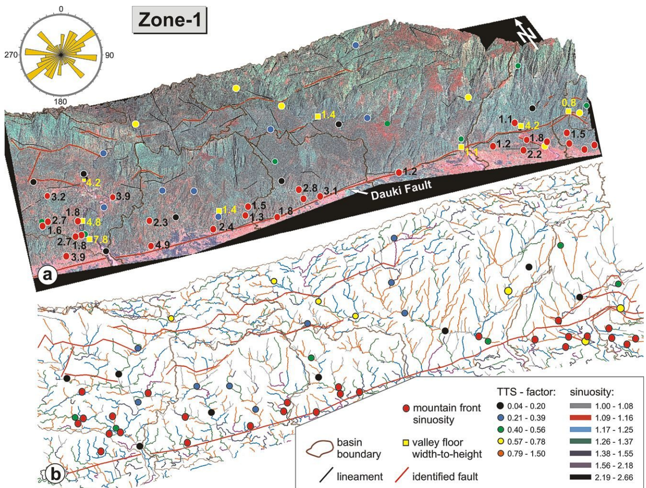
FIGURE 2: Geomorphologic indices and structural features of Zone-1. a) Landsat ETM+ (band 7,4,2 - panchromatic band was used to increase resolution of all bands to 14.5 m) draped on SRTM elevation data (90 m resolutions) with a vertical exaggeration of 3X. Image extent is N25°7'33" to 25°28'52" and E90°32'49" to 91°30'36" b) 3D river network (termed 3D stream profile in text) of Zone-1 displaying the sinuosity of Strahler Stream Order 4 in its colour code with other geomorphologic and structural features. TTS – Transverse Topographic Symmetry.
