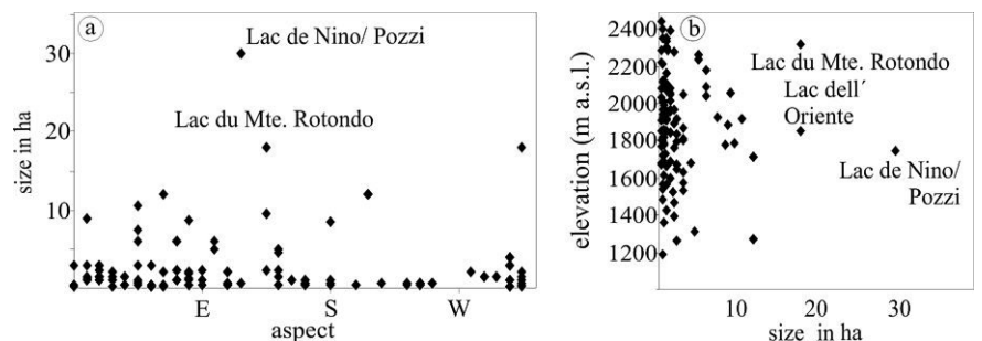
FIGURE 10 A-B: (a) Crossplots of size of glacial depressions vs. elongation aspect; (b) elevation vs. size in ha; (c) crossplot of elongation (length/width) vs. aspect and (d) elevation vs. elongation (length/width).
