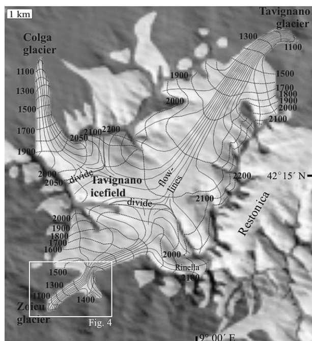
FIGURE 1: Reconstruction of flowlines and divides of the Würmian Tavignano icefield.
