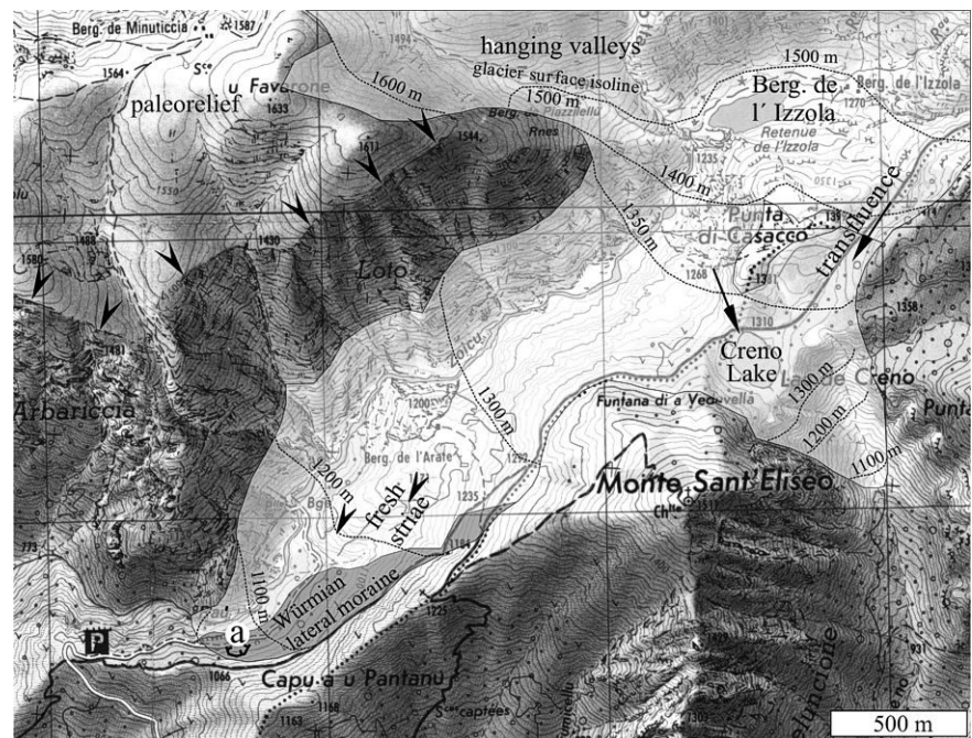
FIGURE 4: Detailed map of the Zoicu valley on the western slope of Haut Tavignano, based on the 1:25000 map IGN 4251 OT. White transparent cover shows the maximum Würmian glacier surface of the western outlet tongue of the Tavignano icefield. At point (a) within the latero-frontal moraine at the end of the Würmian glacier, a fresh open pit exposes brownish oxidised moraine material, containing rhyolite pebbles with perfectly preserved glacial striae. Transfluence from the Zoicu glacier to the small catchment of the Creno Lake is shown by arrows. The former lake at Bergerie de l'izzola, now dry and filled with coarse gravel, exposes a debris cone from the N overlying former swampy meadows.
