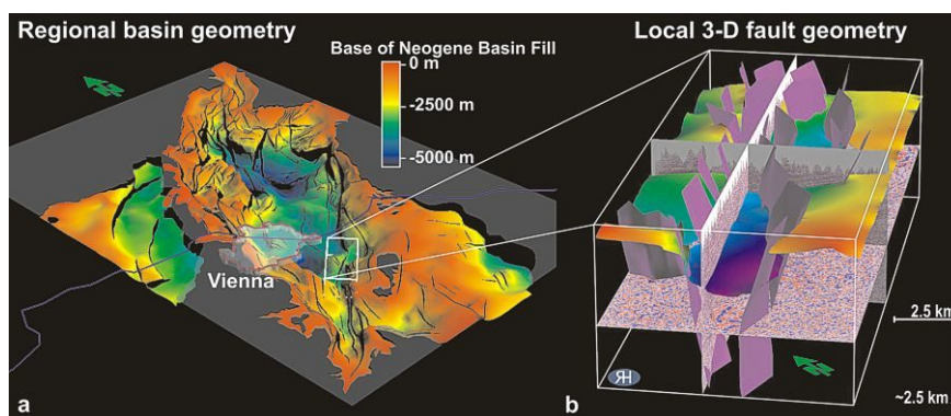
FIGURE 7: (a) 3-D structural model of the Vienna Basin and adjacent areas, based on data from subsurface exploration (Kröll and Wessely, 1993); (b) 3-D structural model from the southern Vienna Basin displaying the complex fault pattern at the southern tip of a pull-apart basin, comprising a negative flower structure and branching normal faults. The mapped faults are tectonically active (Hinsch et al., 2005a). Seismic data with courtesy by OMV, Austria.
