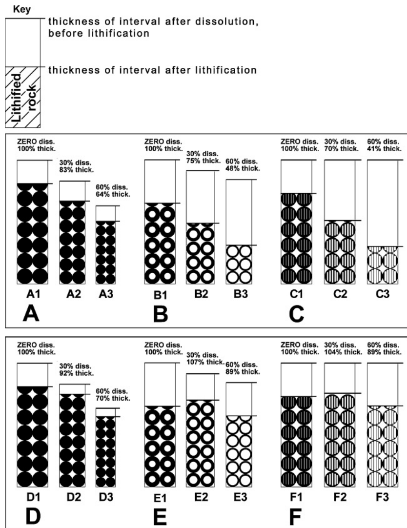
FIGURE 6: Columns of idealized sediments to indicate effect of dissolution loss, cementation and pressure solution on final, lithified layer thickness (LLT). In each column, the upper black line indicates "unlithified" layer thickness after dissolution, the lower black line indicates LLT (zero porosity). Above each column, "diss." indicates percentage dissolution loss, "thick." the percentage of final thickness after full lithification. Each percentage is relative to the column with ZERO dissolution. Case 1 (columns A, B, C): Effect on LLT of dissolution followed by lithification only by pressure solution. A: "Ooids". Dissolution proceeds from the outer grain surface. B: "Dasyclad stems". Dissolution proceeds from both the outer and inner grain surface. C: "Complex bioclasts" with constructional inner cavities. Dissolution proceeds only from the inner cavities. Case 2 (columns D, E, F): Effect on LLT of dissolution followed by cementation of 50% of the pore space, followed by pressure solution (cement is not shown graphically). For comparison, columns D1, E1 and F1 are the same as above, i.e. lithified by pressure solution only. If 50% of the pore space after dissolution is filled by cement, the subtractive effect on LLT is much less. In case of 30% dissolution and 50% reduction of intrinsic pore space by cementation, LLT may exceed that of zero dissolution and lithification only by pressure solution (columns E2, F2). In case of 60% dissolution followed by 50% cementation of the intrinsic pore space, reduction of LLT is comparatively low (columns E3, F3), in particular as compared to lithification only by pressure solution.
