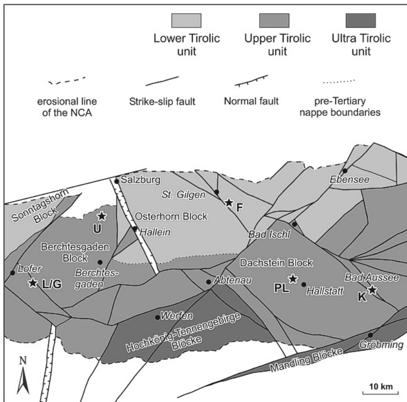
FIGURE 1: Recent tectonic block configuration of the central part of the Northern Calcareous Alps after Frisch and Gawlick (2003) with type-locality of the Plassen Formation (PI) and occurrences of Murania reitneri n. sp., K = Krahstein, L/G = Litzelkogel-Gerhardstein, F = Falkenstein, U = Untersberg.
