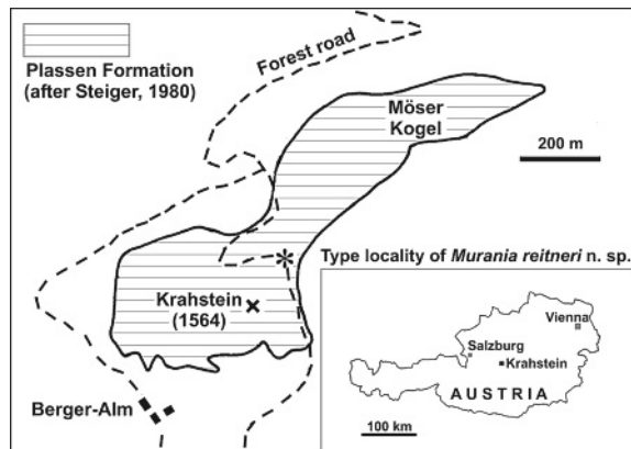
FIGURE 2: Schematic map of the area of the Krahnstein (Styria, Austria) and outcrops of the Plassen Formation after Steiger (1980).
