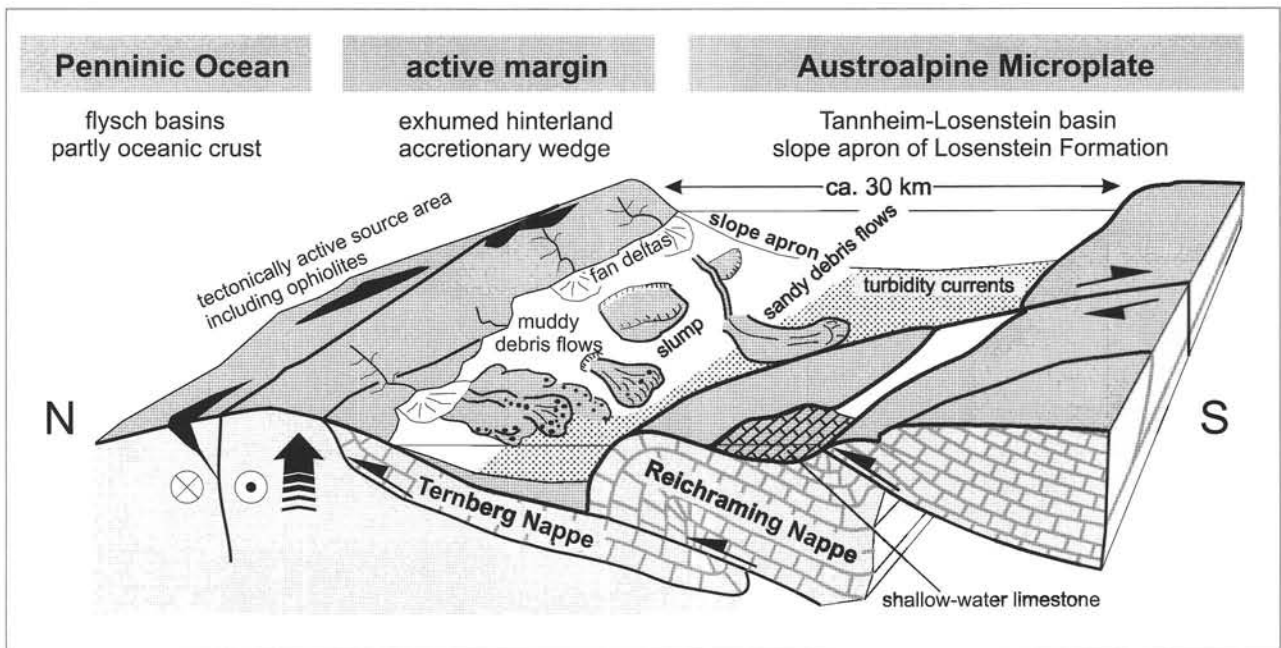
Fig. 9 Slope apron sedimentary systems and piggyback basin model of the Tannheim-Losenstein basin. No east-west differences implied.
