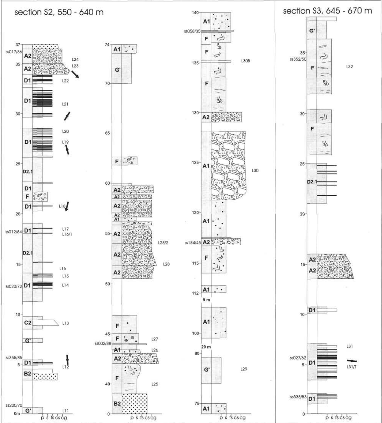
Fig. 6 Type section of the Losenstein Formation (KOLLMANN, 1968), section 2 and 3, southern tributary of the Stiedelsbachgraben east of Losenstein. Arrows indicate unipolar paleocurrent directions (mainly flute casts), lines indicate bipolar paleocurrent data. White areas comprise covered intervals. Grain size scale: p – pelites, s – pelitic slumps, fs – fine sandstone, cs – coarse sandstone, cg – conglomerates. L-numbers indicate sample locations.
