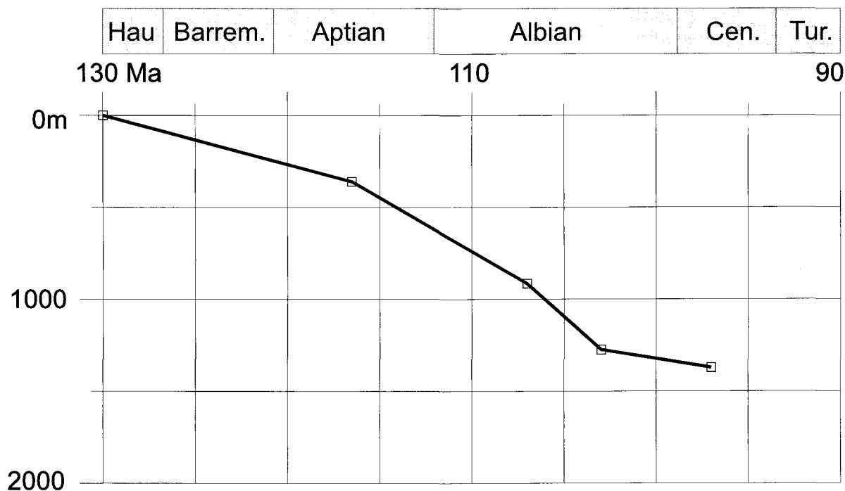
Fig. 11 Backstripped tectonic subsidence curve of the Cretaceous succession of the Losenstein syncline.
