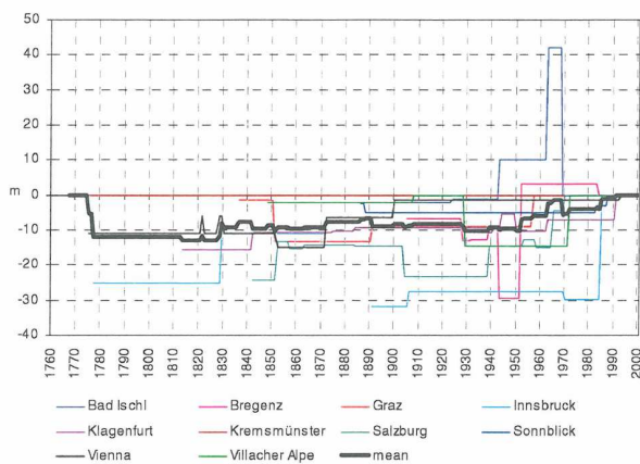
Fig. 4.23. Barometer altitudes relative to actual altitude (old minus new) Thin: single stations, bold: Austrian mean
