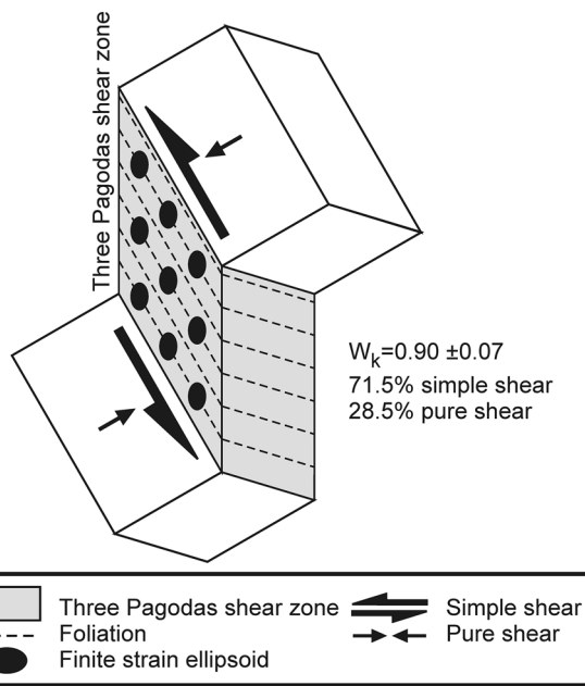
Figure 9: Schematic block diagram illustrating the sinistral ductile deformation within the Three Pagodas shear zone. The values of estimated mean W_k suggest that simple component was predominantly associated with the strike-slip ductile deformation.
