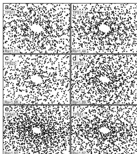
Figure 6: The finite strain ellipses derived from XZ-sections using the nearest neighbour center-to-center Fry method (Fry, 1979). The high-resolution finite strain ellipses of XZ-plane of the samples along the Three Pagodas shear zone; (a) TPS11, (b) TPS14, (c) TPS23, (d) TPS33, (e) TPS41, and (f) TPS51. They commonly present uniform and homogeneous deformation.
