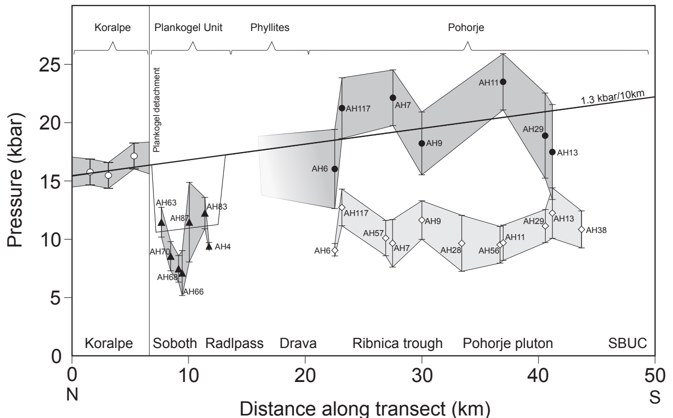
Figure 5: Visual representation of pressure results determined with THERMOCALC along the profile shown in Figs. 1 and 2. The black triangles represent the Plankogel Unit, the black circles represent the peak metamorphic conditions of rocks in the Pohorje area, the white squares represent the decompression conditions of the Pohorje area and the white circles show pressures determined by Tenczer and Stüwe (2003). The transect starts in the Koralpe to the north and ends in the south where the Pohorje mountains dip below the sediments of the Pannonian Basin. The darker shaded area shows the rising pressures from north to south and the lighter shaded area represents the re-equilibrated pressures. The line fitting the peak metamorphic conditions represents the interpreted field gradient discussed in section 5.
