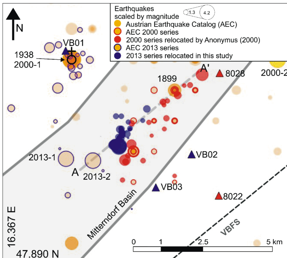
Figure 2: Seismotectonic overview of the area around the VBFS close the Ebreichsdorf. Micone faults from Hinsch and Decker (2011) as solid grey lines. Earthquakes from the Austrian Earthquake Catalog scaled by magnitude (ZAMG, 2014), events mentioned in the text are labeled with year of occurrence. Triangles indicate the positions of seismic stations used in this study. Profile A – A’ parallel to VBFS is used in Figure 4.
