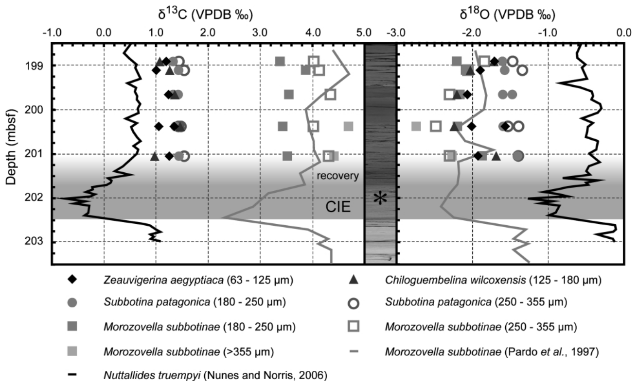
FIGURE 3: Carbon and oxygen isotopes of all measured planktic foraminifers plotted stratigraphically. Additional M. subbotinae data (no size fraction given) from Pardo et al. (1997) and benthic foraminiferal data ( Nuttallides truempyi ) from Nunes and Norris (2006). Note that the dark-colored interval following the CIE of the PETM reflects increased clay content. Asterisk symbol (*) indicates a sample where additional Z. aegyptiaca specimens were studied to check preservation (also see Fig. 4).
