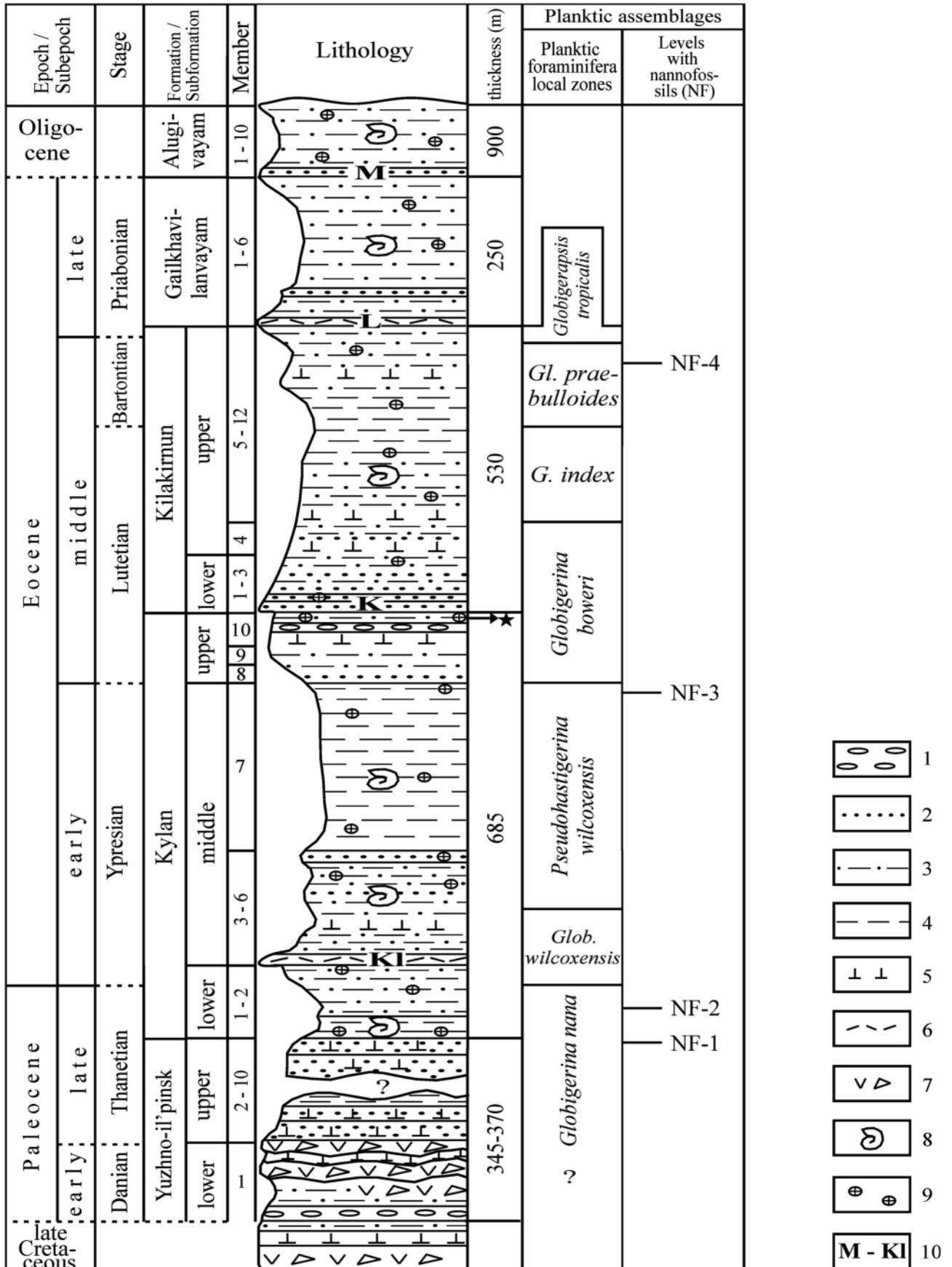
FIGURE 2: Generalized stratigraphic column of the Il'pinskii Peninsula section (after Volobueva et al., 1994; Benyamovskiy, personal communication, 2011), with the position of the diatom-bearing sample from the Upper Kylan Subformation (marked by arrow and asterisk). G. - Globigerapsis , Gl. - Globigerina , Glob. - Globorotalia , 1 – conglomerate, gritstone; 2 – sandstone, tuffstone; 3 – siltstone, argillite, tuffaceous siltstone and argillite; 4 – mudstone; 5 – base and intermediate tuff; 6 – acidic tuff; 7 – lava and lava-breccia; 8 – fossil mollusks; 9 – carbonate concretions; 10 – marker lithological "horizons": the Mulatkhan (M), Laparelam (L), Kilakirnun (K), Kylan (KI).
