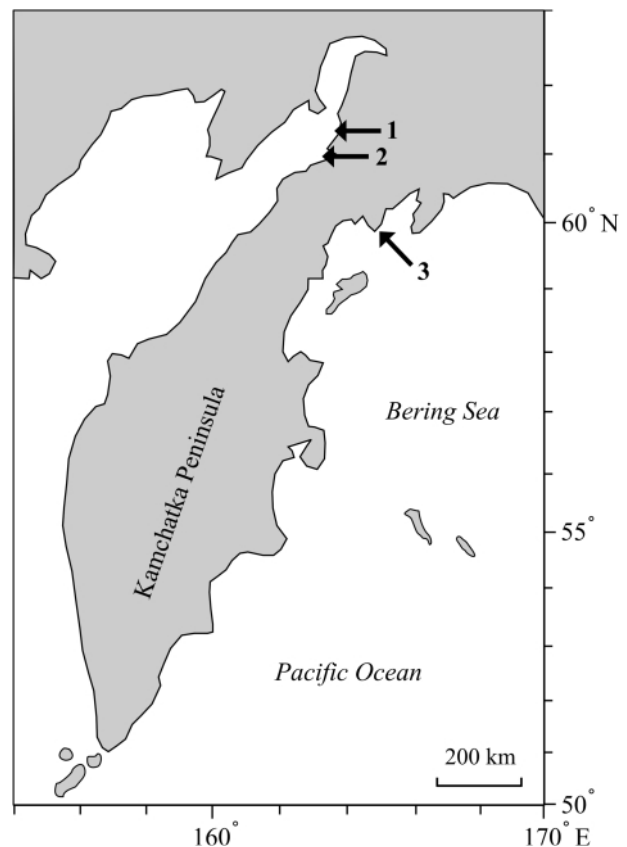
FIGURE 1: Location of the Paleogene stratigraphic key sections (shown by arrows) in North Kamchatka: 1 - the Mametchinsky Bay, 2 - the Chemurnaut Bay, 3 - the Il'pinski Peninsula.
