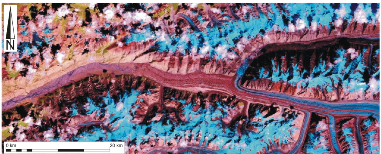
FIGURE 4: Landsat 7 ETM+ of the Inylchek Glacier (acquired August 2006; pan-sharpened; bands 1, 4, 7; ground resolution 15 m. Source: Global Land Cover Facility – GLCF, Maryland/USA).
