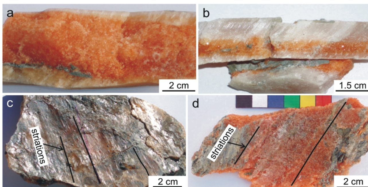
FIGURE 6: (a)–(b) Antitaxial halite veins in mudrock. (c)–(d) Slickensides on wall rock.
