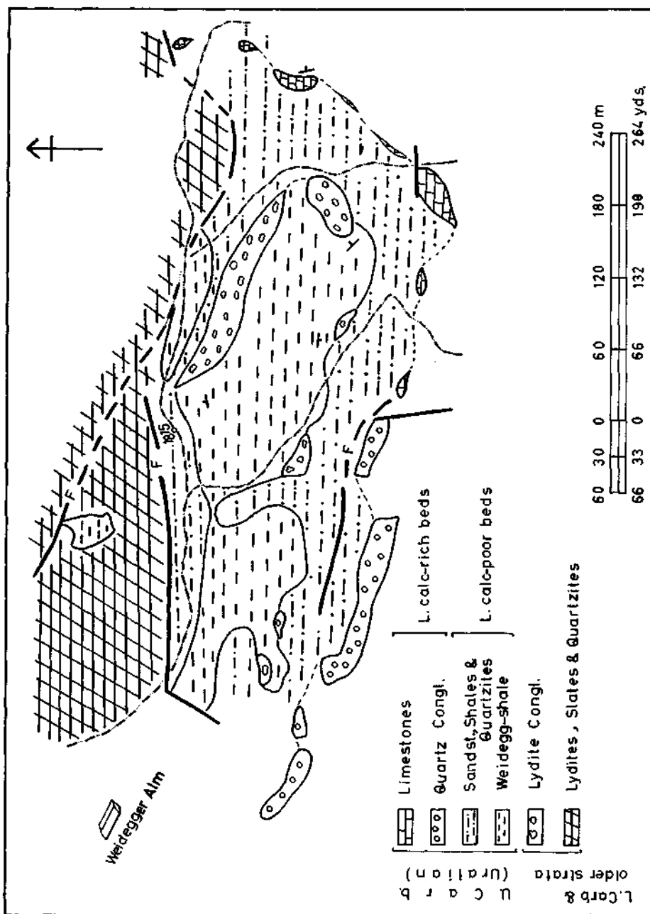
Fig. 2. Geological map of northern part of the Zoelner ridge and neighbourhood.
