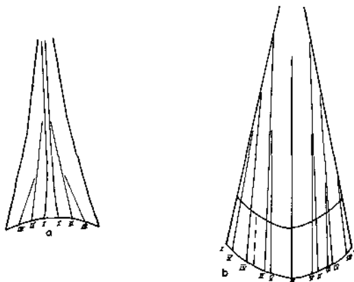
Figs. 22 a, b. Neospirifer lanceolatus n. sp. showing respectively costellation of the ventral sinus and the dorsal fold. \times 3.5 .
