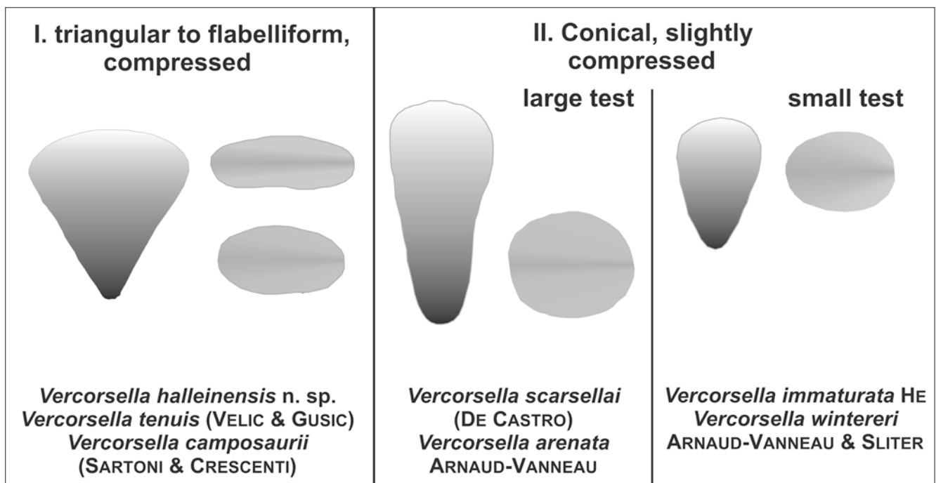
Text-Fig. 4. Test morphology of representatives of Vercorsella ARNAUD-VANNEAU, 1980 allowing the distinction of two major groups, one composed of two subgroups depending on test size and grade of test compression.
