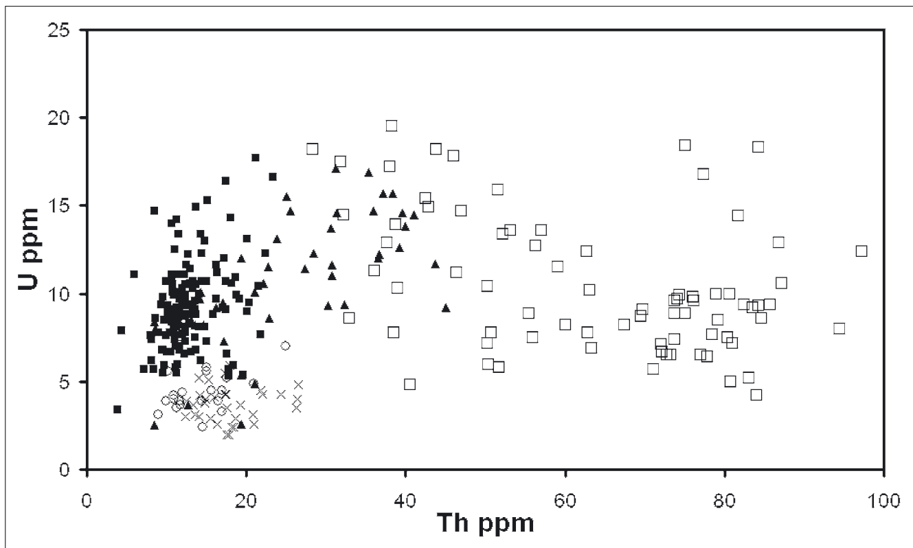
Text-Fig. 2. Contents of Uranium and Thorium in rocks (field spectrometry gamma). □ = Dreiländereck granite; ▲ = melasyenite, ■ = Plöckenstein granite; × = Weinsberg granite, ○ = gneiss.
