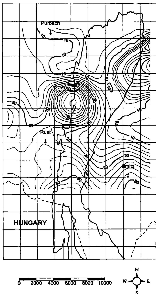
Fig. 1. Magnetic anomaly near Rust
