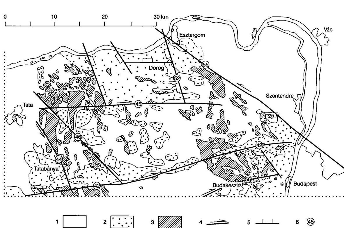
Fig. 1. Eocene and Palaeogene–Miocene fault lines in the DANREG area
