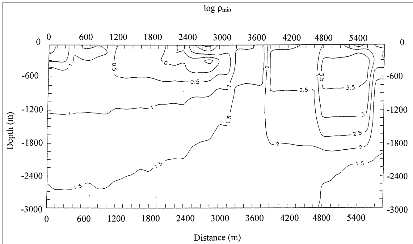
Text-Fig. 9. Two dimensional model of Messern profile. \log(\rho_{\min}) [Ωm] as function of distance [m] and depth [m]. Isolines: \log(\rho_{\min}) .
