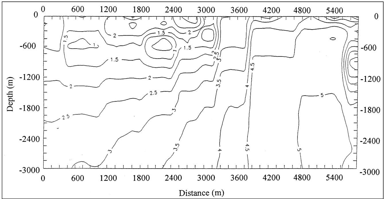
Text-Fig. 10. Two dimensional model Messern profile. \log(\rho_{\max} [\Omega\text{m}]) as function of distance [m] and depth [m]. Isolines: \log(\rho_{\max}) .
