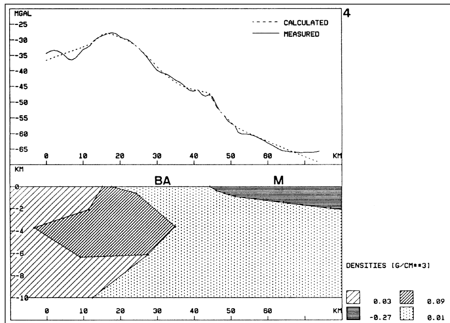
Text-Fig. 14. Two-dimensional model of the upper crust of the Southern Bohemian Massif. Profile 4 (marked in Plate 2, top). BA = Bavaricum ( 2.68 \text{ gcm}^{-3} ); M = Molasse ( 2.40 \text{ gcm}^{-3} ).
