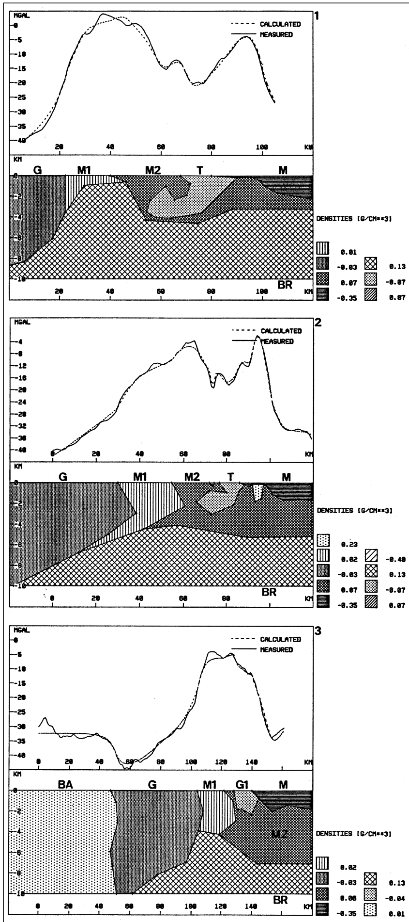
Text-Fig. 13. Two-dimensional model of the upper crust of the Southern Bohemian Massif. Profiles 1-3 (marked in Plate 2, top). BA = Bavaricum ( 2.68 \text{ g cm}^{-3} ); BR = Brunovistulicum ( 2.80 \text{ g cm}^{-3} ); G = Granite intrusion ( 2.64 \text{ g cm}^{-3} ); G1 = Granulite ( 2.63 \text{ g cm}^{-3} ); M = Molasse ( 2.32 \text{ g cm}^{-3} ); M1 = Moldanubicum ( 2.69 \text{ g cm}^{-3} ); M2 = Moldanubicum + Moravicum ( 2.74 \text{ g cm}^{-3} ); T = Thaya batholite ( 2.60 \text{ g cm}^{-3} ).
