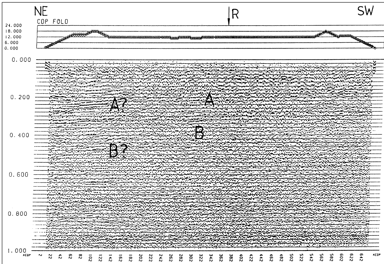
Text-Fig. 7. Final brute stack of Nondorf profile. Abscissa: CMP-number, CMP-distance = 5 m; ordinate: two-way-travel time [s]; A, B, C = events; R = intersection of Messern profile. Top: graph of the CMP fold.
