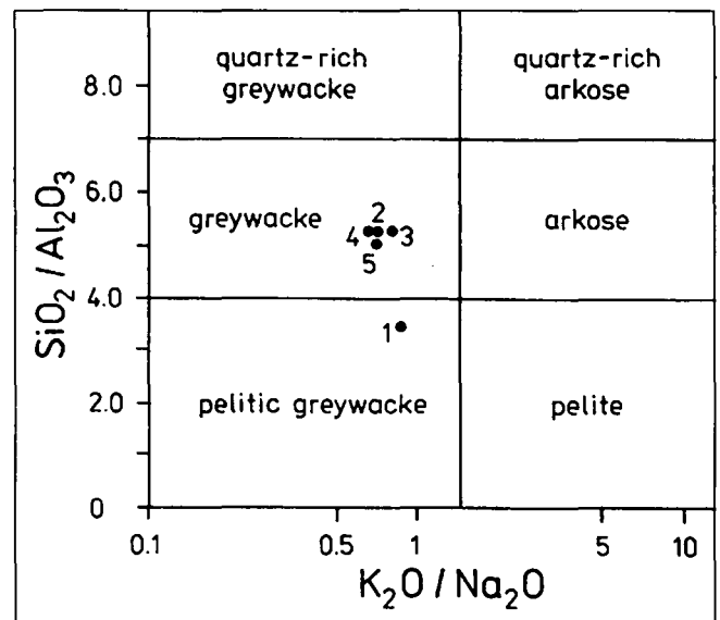
Text-Fig. 2. Greywackes of the Andělská Hora Fm. in the K_2O/Na_2O versus SiO_2/Al_2O_3 ratios plot for clastic sediments after WIMMENAUER (1984). The sample numbers from Table 2 are given with the symbols.
