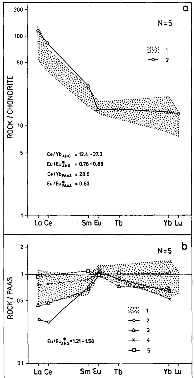
Text-Fig. 5. a) REE distribution in the Andělská Hora Fm. greywackes (AHG) normalized to average chondrite REE abundances (HERRMANN, 1970) (1); for the comparison chondrite-normalized post-Archean Australian average shale (PAAS) REE concentrations after TAYLOR & MCLENNAN (1985) are shown (2). b) REE distribution in the Andělská Hora Fm. greywackes (AHG) normalized to the PAAS lanthanide abundances (TAYLOR & MCLENNAN, 1985) (1); for comparison the PAAS-normalized REE distribution curves for greywackes of various tectonic settings – oceanic island arc (2); continental island arc (3); Andean-type continental margin (4) and passive continental margin (5) – are presented (BHATIA, 1985).
