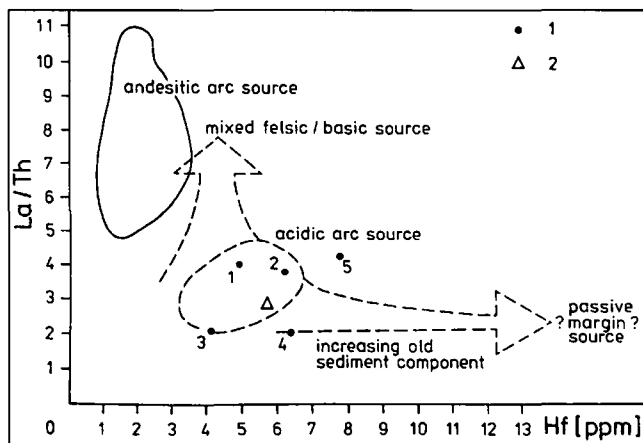
Text-Fig. 8. The Andělská Hora Fm. greywackes in the Hf versus La/Th diagram for source and compositional discrimination of clastic sediments (FLOYD & LEVERIDGE, 1987).
