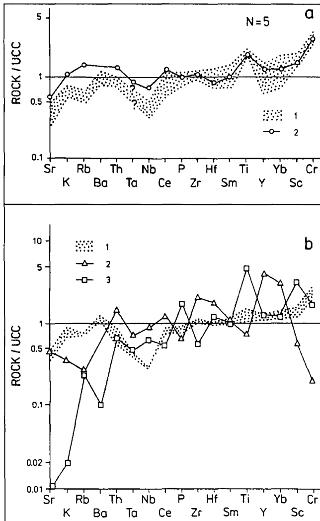
Text-Fig. 4. a) Trace element distribution in the Andělská Hora Fm. greywackes relative to upper continental crust composition after TAYLOR & MCLENNAN (1985) (1); for comparison the post-Archean average shale trace element abundances (identically normalized) (TAYLOR & MCLENNAN, l.c.) are presented (2). The elements are arranged according to PEARCE (1982). b) Trace element distribution in potential source rocks of Andělská Hora Fm. greywackes – Orlik nappe Group metamorphics (one metagranite blastomylonite and two mica schists) (1); Devonian Rejvíz Group porphyroid (2) and Devonian Vrbno Group greenschist (3) – relative to upper continental crust composition after TAYLOR & MCLENNAN (1985). The elements are arranged as in (a).
