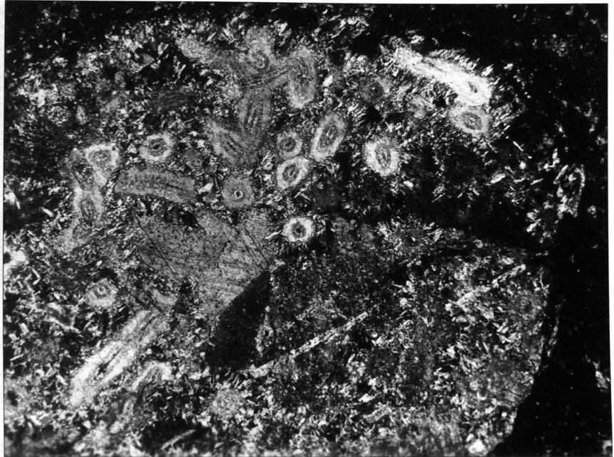
Text-Fig. 3. Xenolith of organic-detritic limestone (Liasic?) in alkaline basalt. Nizke Tatry Mts. Enlargement 95x.
