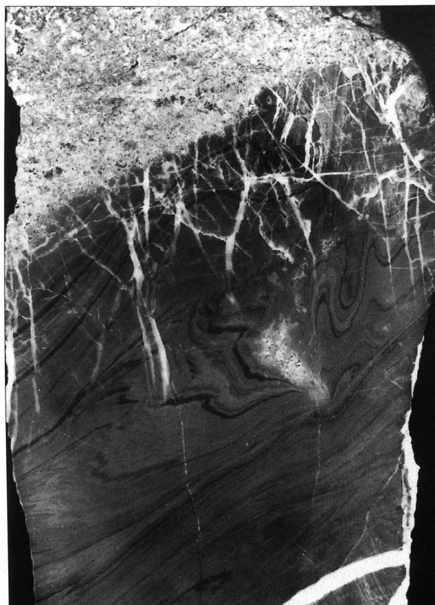
Text-Fig. 6. Plastic deformation of not yet lithified carbonate mud by moving basaltic magma. Epigenetic cracks are filled up by calcite. Vel'ká Fatra Mts. Polished surface. Enlargement 1,5×.
