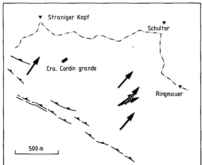
Fig. 7: Paleoflow directions of the Auernig Group, trending normal to the reverse fault. The beginning of the arrow indicates the situation of the outcrop.
