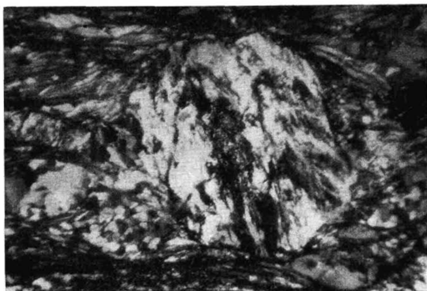
Fig. 4. Quartz-albite-muscovite-chlorite schist. Porphyroblastic albite showing post-crystalline rotation. Inclusions are mainly of graphite. Section parallel to N-S, L 1 -lineation (Fuchsloch, N.-O.).
