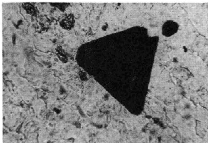
Photo 7. Triangular section of magnetite from the marginal zone of riebeckite gneiss ( \times 350 ).
