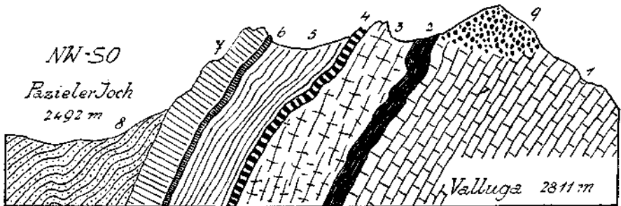
Fig. 23. 1 = Hauptdolomit. 2 = Kössener Schichten. 3 = Oberrätalkalke. 4 = roter Liaskalk. 5 = Fleckenmergel. 6 = roter, 7 = grauer Tithonkalk. 8 = Kreideschiefer. 9 = Eisenspitzebreccie (Gosau?)
