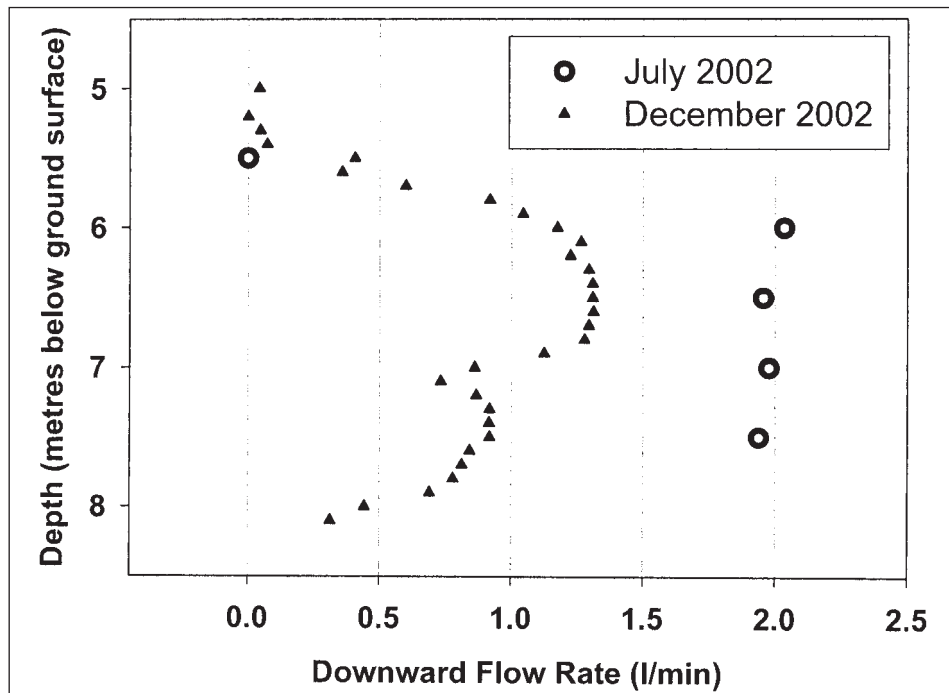
Fig. 6: Downward flow rates in K3-2, Kappelen Test Site, Switzerland, measured using heat pulse flow meter in July 2002 and December 2002.
