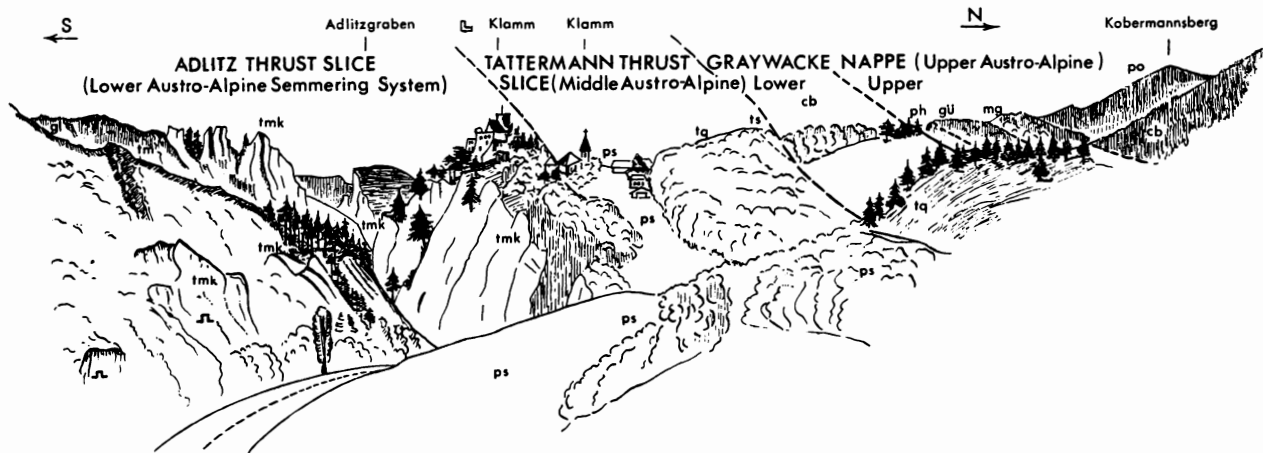
Fig. 2. View of the northern border of the Semmering system near Klamm, seen from Aue towards west (abbr. as in plate 1) (A. TOLLMANN, 1966).
