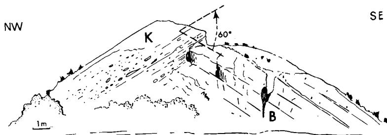
Fig. 5. Outcrop of pisplitic, bauxitic clay (B) and of unconformably overlying Maestrichtian conglomerate (K) at Alland.
