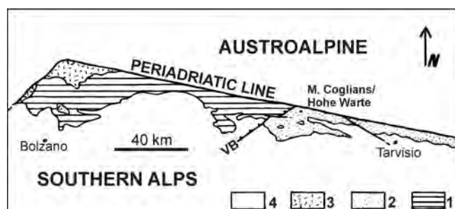
Figure 2. Simplified geological map of the Southern Alps showing the partition of the Palaeocarnic Chain into a West and an East Zone (after Venturini & Spalletta, 1998, modified). VB: Val Bortaglia thrust. 1. Low to middle grade metamorphic basement. 2. Non- to anchi-metamorphic units. 3. Variscan intrusive bodies; 4: post-Palaeozoic units.
