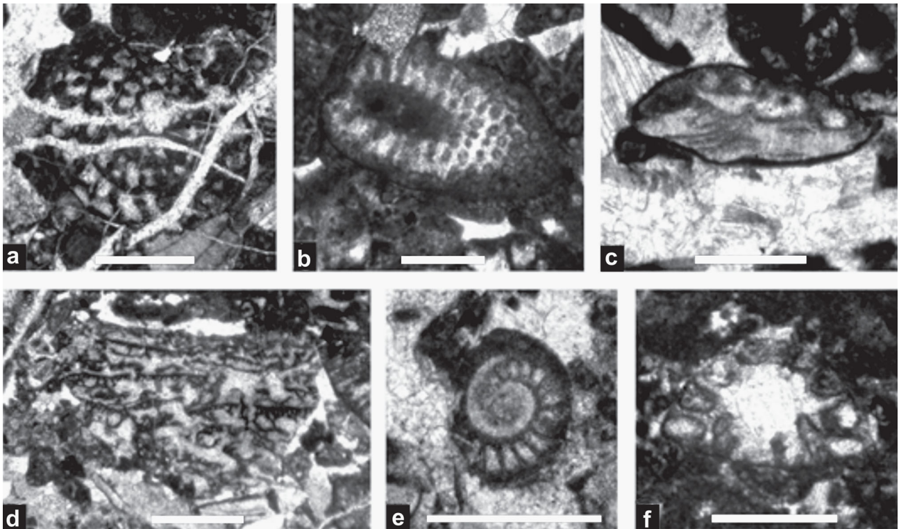
Fig. 4. Microfossils of the Kimmeridgian allodapic limestones (sample GS132). a — benthic foraminifer Labyrinthina mirabilis Weynschenk, b — Dasycladale Salpingoporella pygmaea (Gümbel), c — benthic foraminifer Mohlerina basiliensis (Mohler), d — incertae sedis Pseudolithocodium carpathicum Misik, e — benthic foraminifer Protopenneroplis striata Weynschenk, f — benthic foraminifer Coscinoconus cf. alpinus Leupold. Scale bars = 0.5 mm.
