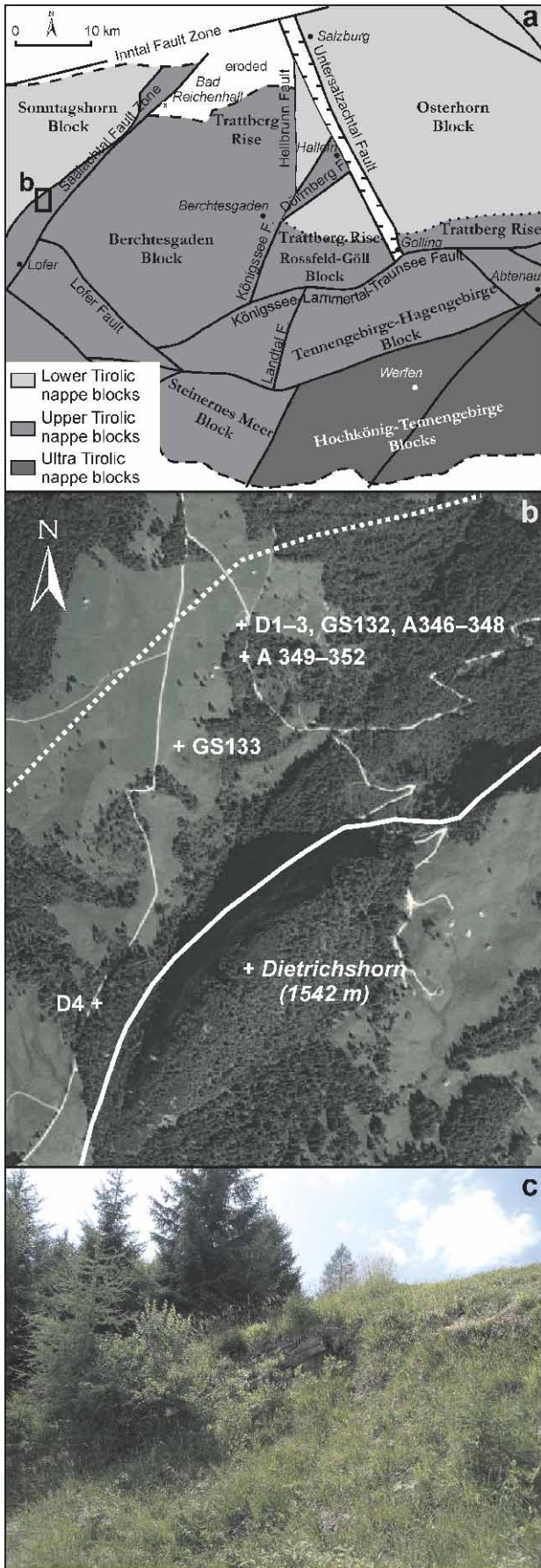
Fig. 2. a — recent block configuration of the western part of the central northern Calcareous Alps with major faults active during Miocene lateral tectonic extrusion after Frisch & Gawlick (2003) and study area; b — position of the sampling sites. Topographic background photo from Google Earth (2014). The white line should mark the boundary between the Upper Jurassic shallow-water platform carbonates of Mount Dietrichshorn and the Lower Cretaceous sedimentary rocks to the west and is interpreted as a normal fault according to Ortner et al. (2008). In fact the dotted line is the thrust plane of Mount Dietrichshorn above the Sillenkopf Formation. All Kimmeridgian samples plot into this area. The strike-slip fault separating the Sillenkopf Formation from the Lackbach Formation must be located in the northeastern grassland area (dotted line). See text for explanation; c — outcrop situation in the year 2012. The artificial digging from the year 2006 (first sampling campaign) is mostly covered. Along the forest road several similar outcrops exist, with the same dipping below Mt Dietrichshorn (eastward). In contrast, the Lackbach Formation shows a westward dipping.
