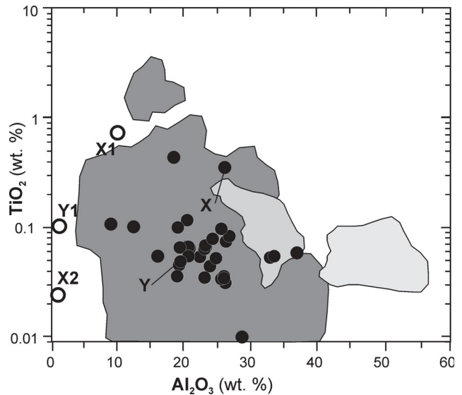
Fig. 11. Dietrichshorn spinels plotted in the TiO 2 vs. Al 2 O 3 diagram and compared with spinel chemistry from the West-Carpathian Cretaceous synorogenic sediments (dark grey field, diagram from unpublished data of Jablonský et al. 2001) and Meliatic and Penninic primary ophiolitic outcrops (light-grey fields, data from Mikuš & Spišiák 2007).
