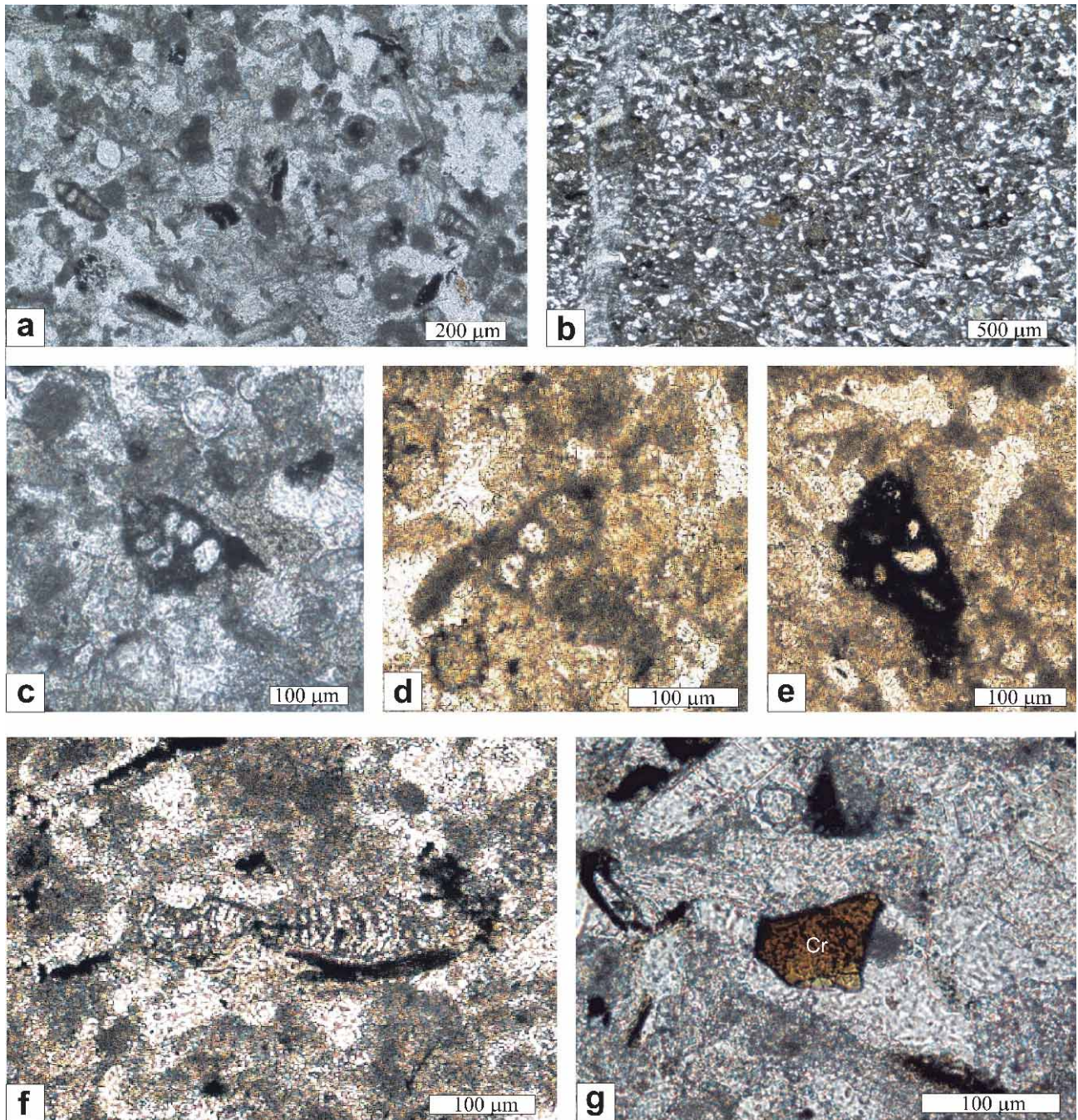
Fig. 6. Microfacies of the sampled silicified allodapic limestones. a — well-sorted organodetrital sediment forming the main portion of the examined allodapic limestones, b — parts of the rocks representing the fine-grained matrix consist of spiculitic-radiolarian microfacies, c-e — Textulariids are the most common foraminifers in the sediment, f — Spirillina sp. Cr — detritic chrome spinel grain.
