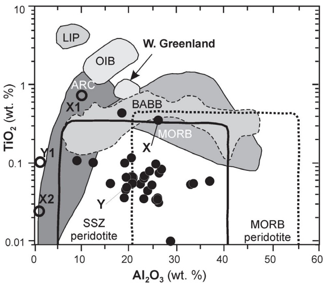
Fig. 10. Dietrichshorn spinels plotted in the TiO 2 vs. Al 2 O 3 diagram of Lenaz et al. (2000) and Kamenetsky et al. (2001). Explanations: LIP — large igneous provinces, OIB — ocean island basalts, ARC — island-arc magmas, BABB — back-arc basin basalts, MORB — middle ocean ridge Basalts, SSZ — supra-subduction zone peridotites, full circles — fresh spinels, empty circles — altered spinel rims.
