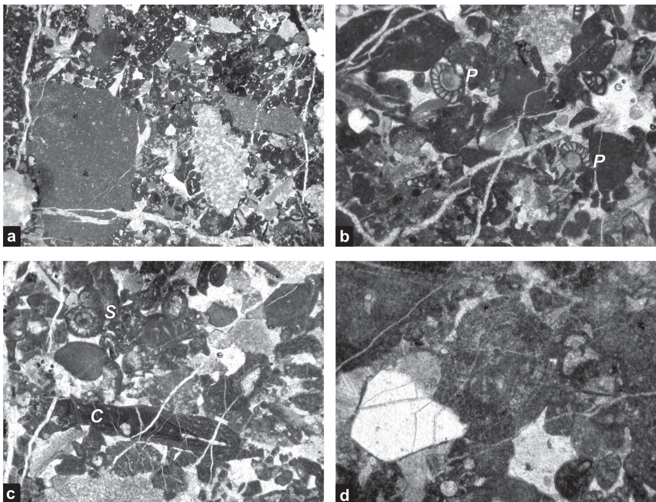
Fig. 5. Microfacies of the studied allodapic limestones (samples GS132, A346–352). a — poorly sorted packstone with benthic foraminifera, debris of corals and a large radiolarian wackestone lithoclast, which resembles the basalinal microfacies of the Sillenkopf Formation. Width of photo: 1.4 cm; b — magnified view of a grain-/packstone with two specimens of Protopeneroplis striata Weynschenk. Width of photo: 0.5 cm; c — grain-/packstone with incertae sedis Crescentiella morronensis (Crescenti) (C) and dasycladale Salpingoporella pygmaea (Gümbel) (S); Width of photo: 1.4 cm; d — magnified view with ooids and a subangular quartz grain. Width of photo: 0.25 cm.
