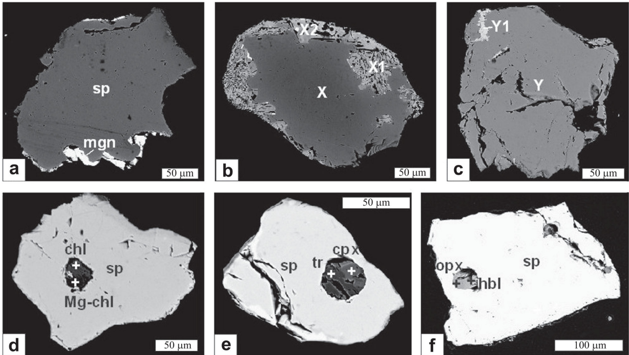
Fig. 7. a–c — photographs of spinel grains with altered rims. Abbreviations: sp — spinel, mgn — magnetite, X, X1, X2, Y, Y1 — measurement points corresponding to the measurements plotted in the diagrams of Fig. 4 and Fig. 6; d–f — examples of inclusions in spinel grains. Explanations: chl — chlorite, Mg-chl — clinochlore, tr — tremolite, cpx — clinopyroxene, opx — orthopyroxene, hbl — hornblende.
