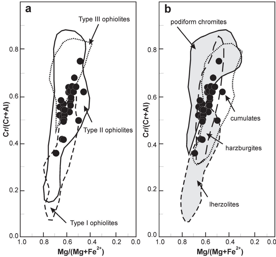
Fig. 9. a — Dietrichshorn spinels plotted in the Cr/(Cr+Al) vs. Mg/(Mg+Fe 2+ ) diagram with fields distinguished by Dick & Bullen (1984). The vertical distribution of the points best matches to the type II ophiolites; b — the same measurements plotted in the diagram with the fields distinguished by Pober & Faupl (1988). In this diagram, the vertical distribution best matches the field of harzburgites.
