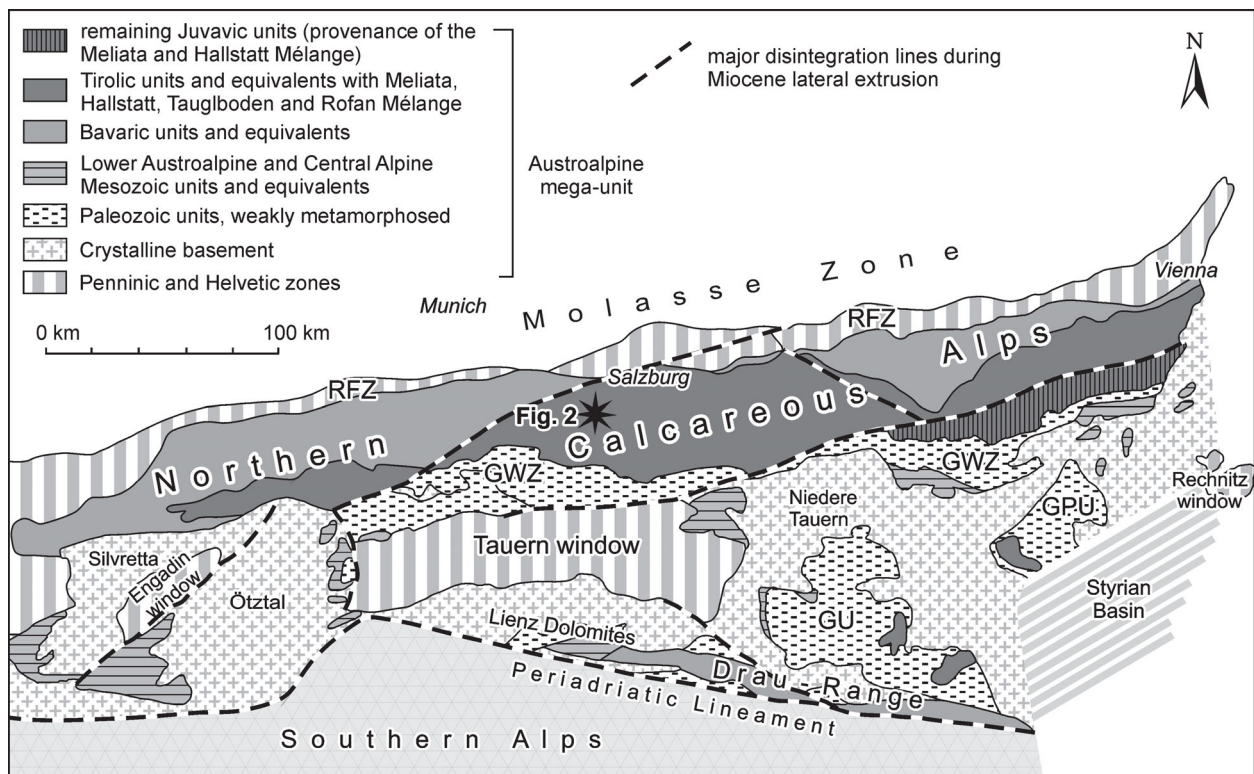
Fig. 1. Tectonic sketch map of the Eastern Alps and study area (black star) southwest of Salzburg (after Tollmann 1977; Frisch & Gawlick 2003). GPU — Graz Paleozoic Unit, GU — Gurktal Unit, GWZ — Greywacke Zone, RFZ — Rhenodanubian Flysch Zone.
