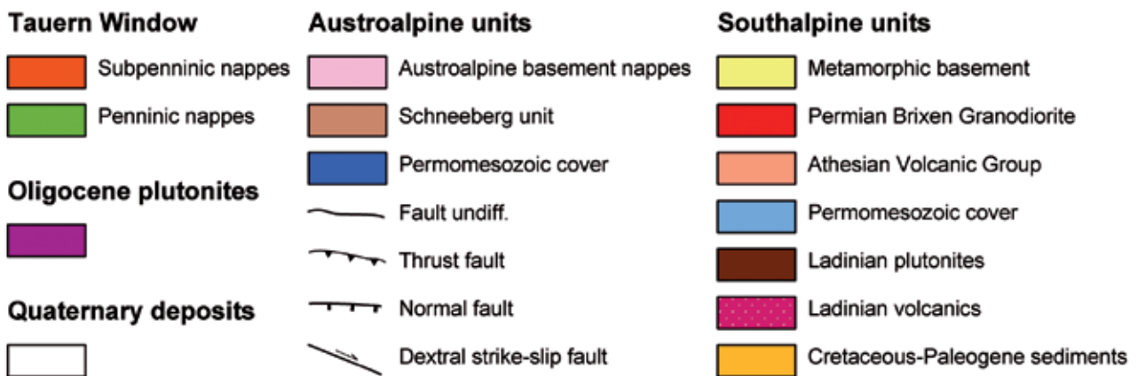
Fig. 1: Regional geologic overview with location of the excursion area in the Dolomites (rectangular).
