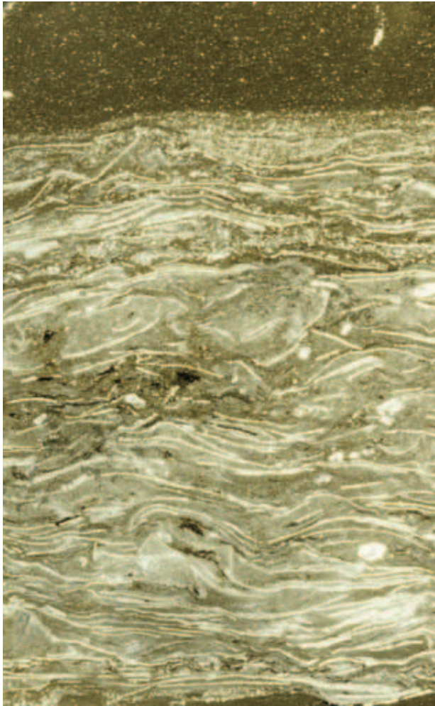
Fig. 11: Thin section photomicrographs of typical tempestite beds with grading and coquinas with Claraia clarai (after Brandner & Keim, 2011).
