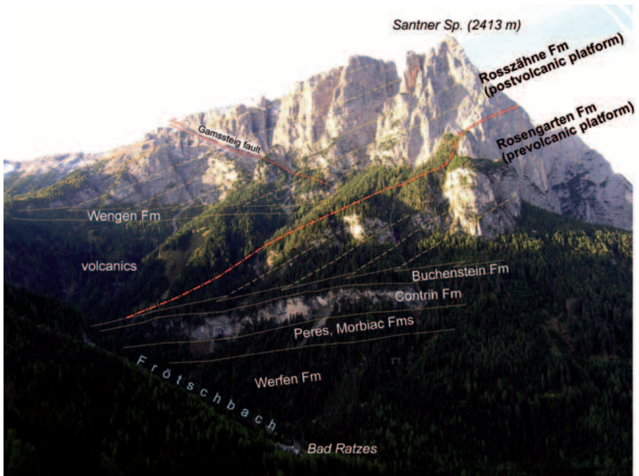
Fig. 15: Panoramic view on the north-eastern flank of the Schlern showing the excellently preserved, seismic-scale platform-to-basin transition of the Anisian to Ladinian carbonate platform. Depositional sequences are bordered by 3 rd order unconformities (stippled lines).
