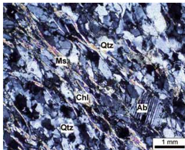
Figure 6: Photomicrograph of the mineral assemblage of the Wildschönau Schists containing muscovite (Ms), quartz (Qtz), albite (Ab) and chlorite (Chl) (sample A-101, X Nicols).
