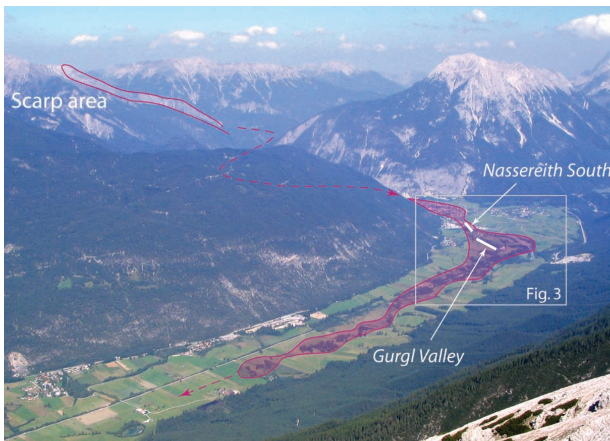
Fig. 2: Oblique view towards northeast to the upper Gurgl valley and the Nassereith area showing the scarp area and the distribution of the Fernpass rockslide deposits. Stippled lines indicate the deflected accumulation path of the southern Sturzstrom branch.
