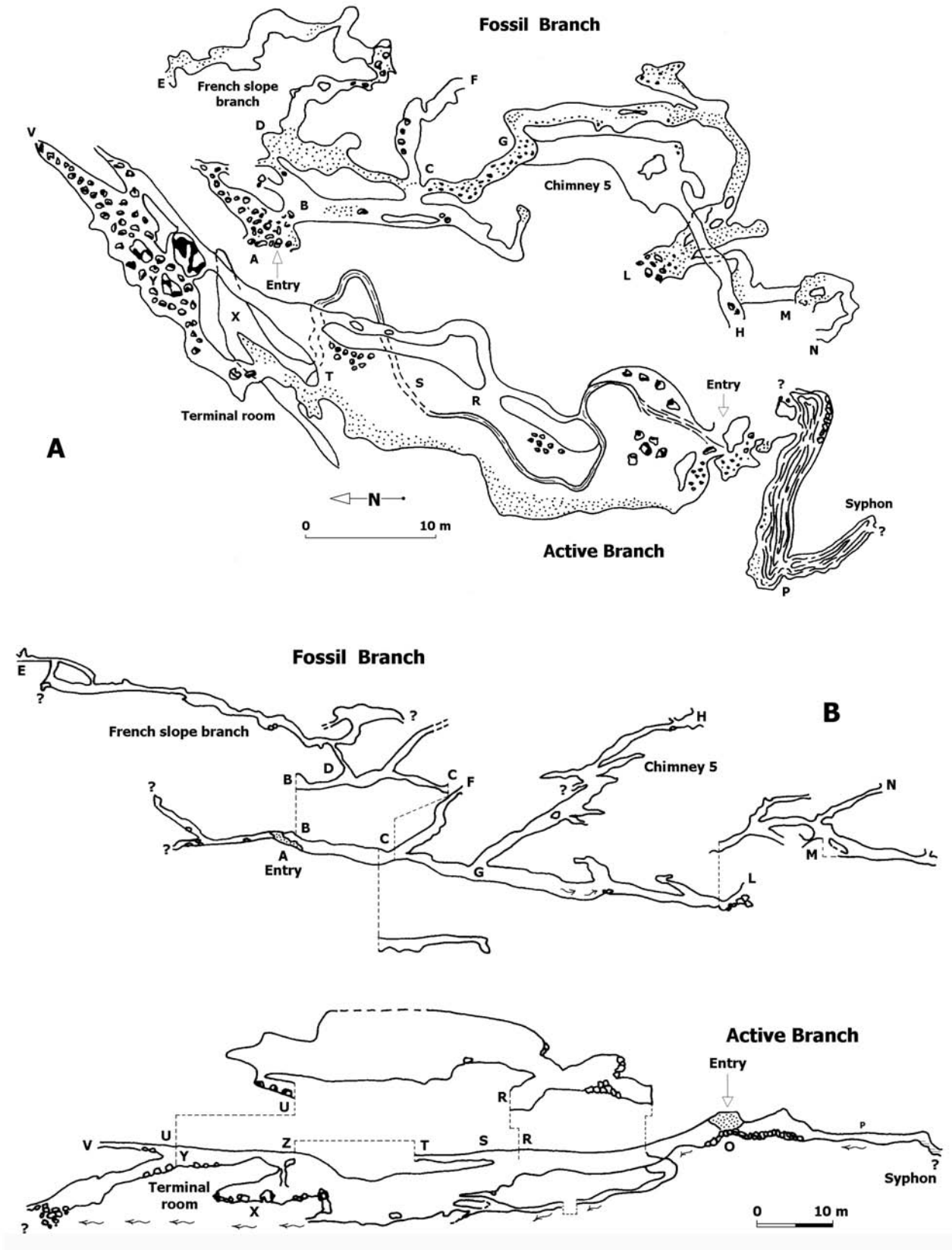
Fig. 2: A – Planimetric scheme and profiles; B – of the Delle Streghe Cave (Cella, 1993, mod.).
