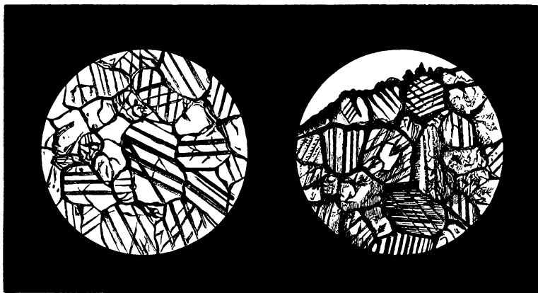
Fig. 1. —Microscopic structure of white marble employed in Edinburgh tombstones. A, Structure of the fresh marble. B, Structure of the marble after standing eighty-seven years. The black edge is the crust of sulphate of lime and town dust which descends along rifts and cleavage planes.
