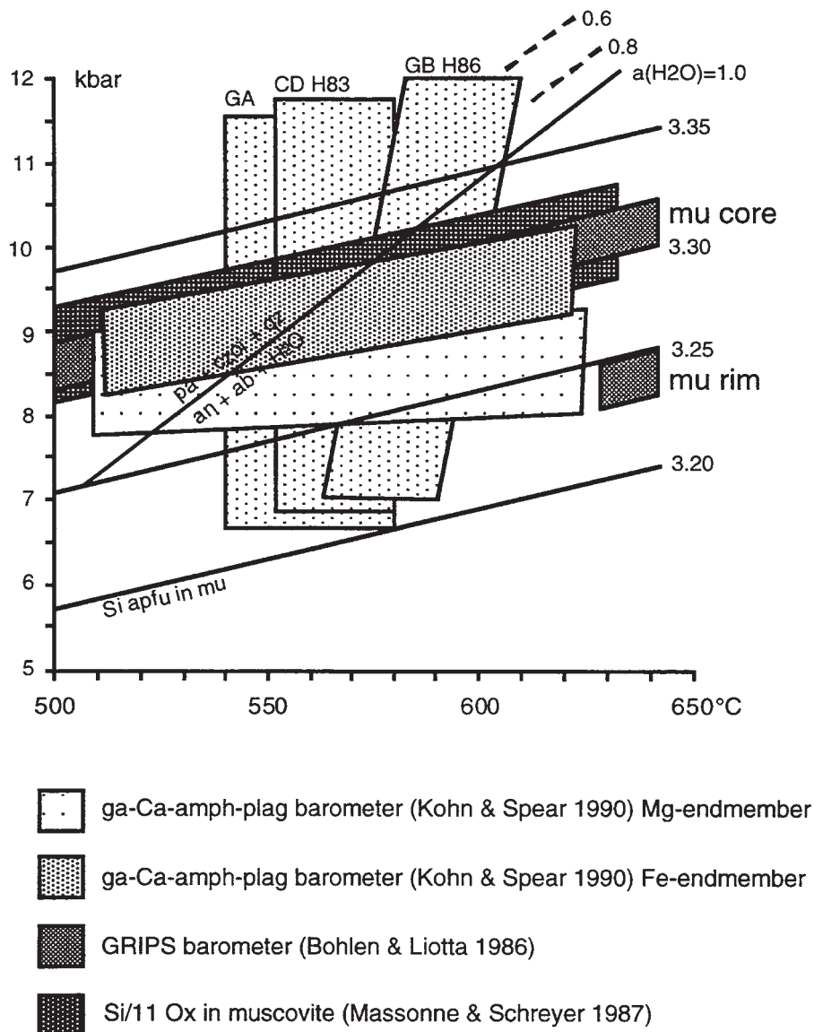
Fig. 6: P-T conditions of metamorphism derived from various geothermobarometers for paragonite amphibolites of the central Schneeberg Complex. GA: garnet-Ca-amphibole thermometer (Graham & Powell 1984); CD H83: results of calcite-dolomite thermometry (Hoinkes 1983); GB H86: results of garnet-biotite thermometry (Hoinkes 1986)
