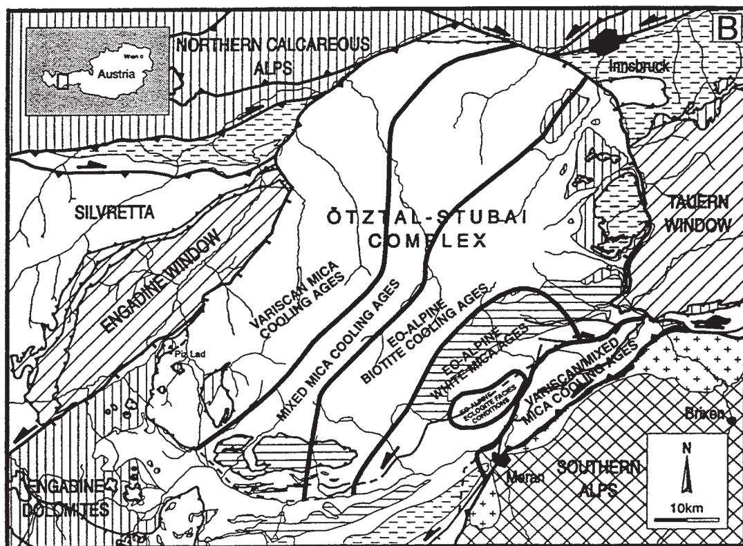
Fig. 4: Sketch of mica cooling age patterns in the ÖSCC resulting from Eo-Alpine overprint of Variscan assemblages (Taken from Elias 1998); figure caption as for Fig. 1.
