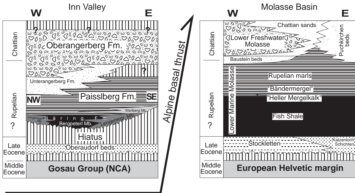
Fig. 3: left side: Lithostratigraphy of the Oligocene in the Inn Valley (modified from Ortner, 1996); right side: Facies development of the Oligocene of the German Molasse Basin (modified from Bachmann & Müller, 1991).
