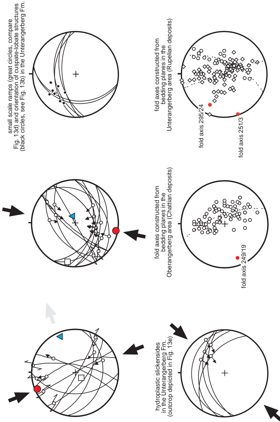
Fig. 14: Orientation of tectonic structures in the Unterangerberg- and Oberangerberg area.
