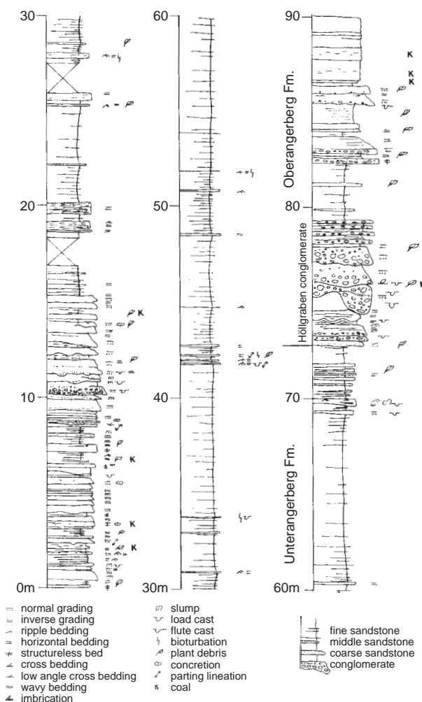
Fig. 15: Section Kleinsöll: Reference section for the upper boundary of the Unterangerberg Fm., and the base of the Oberangerberg Fm. (Hüllgraben conglomerate) at stop 8.
