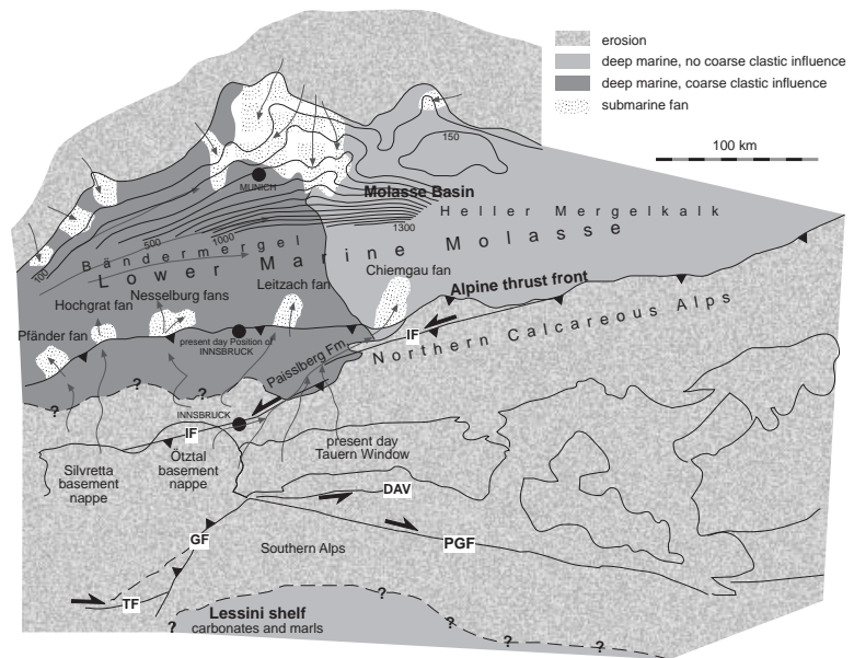
Fig. 10: Paleogeographical sketch of the Eastern and Southern Alps during the Middle Rupelian, at the transition from transgressive to highstand systems tract in Molasse Basin ("Heller Mergelkalk" = condensed section). Isolines in northern part of Molasse basin indicate increase of thickness of Rupelian deposits to the south. Alpine nappes are taken back to a possible Rupelian position following Freudenberger & Schwerd (1996). Major active faults at approximately 33 Ma: IF...Inntal shear zone (this study), TF...Tonale fault, GF...Giudicarie fault, DAV...Defreggen-Antholz-Vals line, PGF...Pustertal-Gailtal fault (Mancktelow et al. 1999). Most of the area of the Alpine orogen was subject to erosion. Generally, during the Early Oligocene the sedimentary cover of the central Alpine basement units was eroded.
