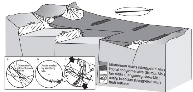
Fig. 7: Block diagram of the Inntal area during deposition of the Häring Fm. WNW-trending dextral faults dissected the area and formed half-graben shaped small restricted basins. Inset: a) Orientation of neptunian dykes filled by flowstones and debris from Werlberg Mb., b) WNW-trending dextral faults sealed by the Werlberg Mb. of the Paissberg Fm., c) brittle fault plane data set compatible with a) and b) indicating NNW-SSE directed compression.
