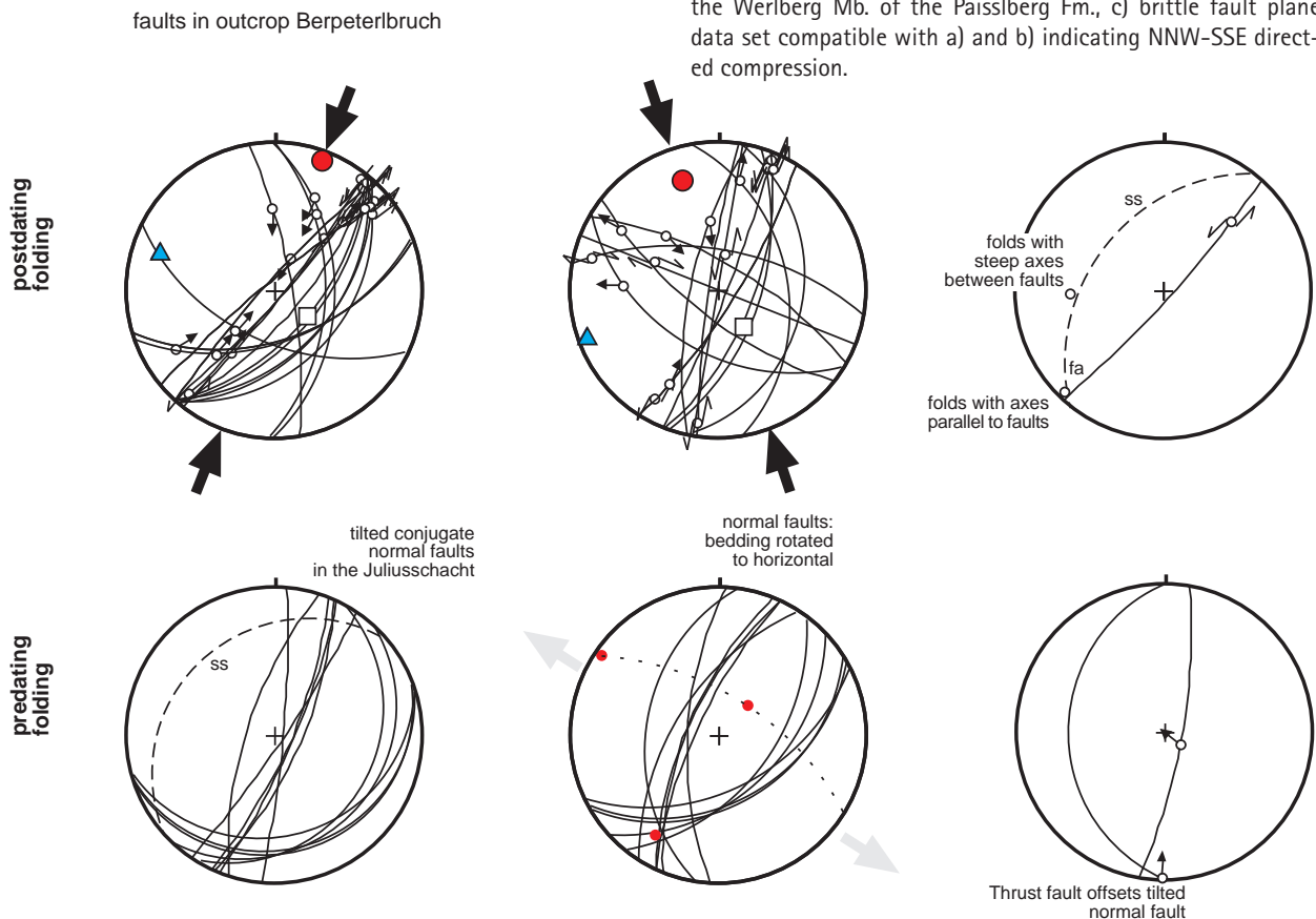
Fig. 8: Faults in the outcrop Bergpeterlbruch, steps 3 & 4. Tilted normal faults predate folding of Oligocene rocks and can possibly be seen in connection with Oligocene sinistral shearing in the area (see also stop 7). Dextral and sinistral shearing postdates folding, and in map view sinistral faults offset dextral faults.
