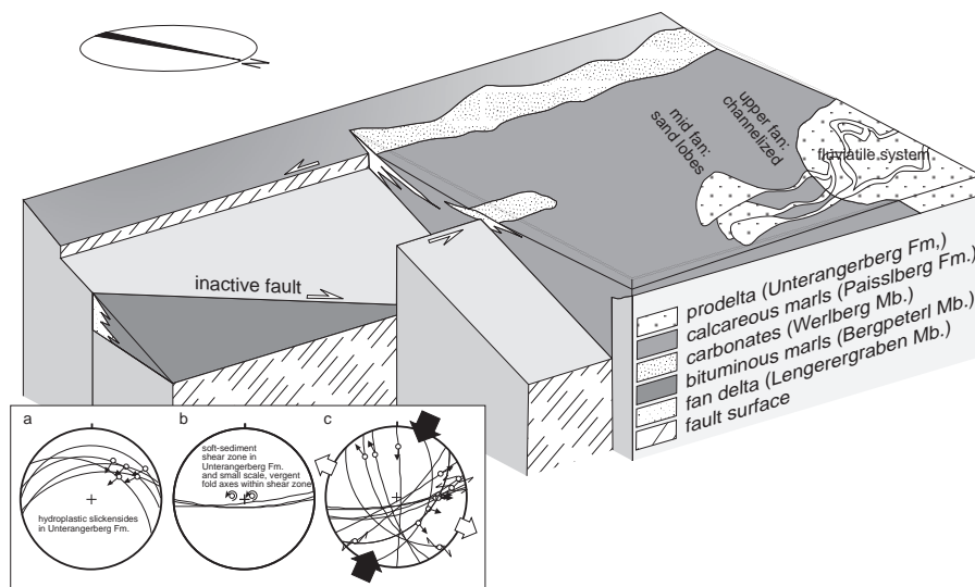
Fig. 12: Block diagram of the Inntal area during deposition of the Paisslberg and Unterangerberg Formations. Werlberg Mb. rims the southern margin of the basin and isolated horsts inside the basin. Fault blocks between active sinistral faults show half graben geometry. From the west, a fluvial system approaches, with the Unterangerberg Fm. in a prodelta position. Inset: a) Top SW reverse faults with hydroplastic slickensides indicating activity before final lithification, b) shear planes in pseudoductile shear zone (great circles) and small scale fold axes with vergence of folds indicating a sinistral shear sense, c) brittle fault plane data set compatible with b) indicating NNE-SSW compression.
