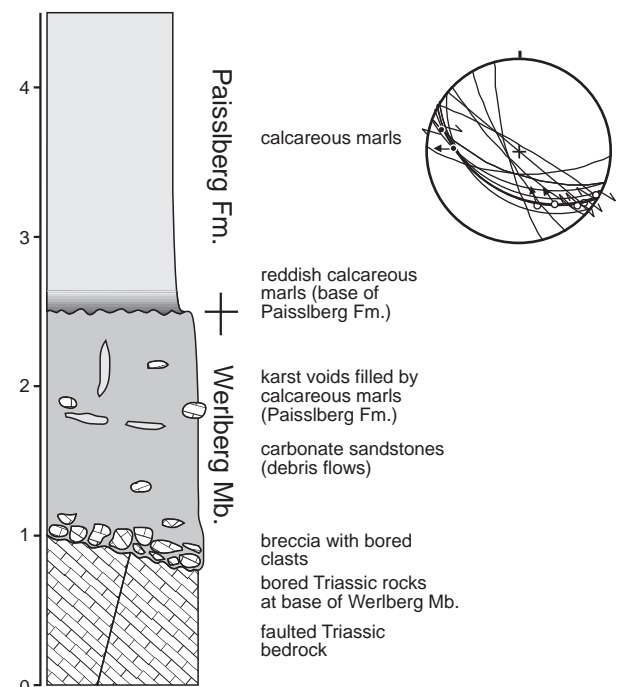
Fig. 4: section of the Werlberg Mb. at stop 1. Above: Orientation of neptunian dykes, sealed faults (open symbols) and faults sealed by neptunian dykes (black symbols).
