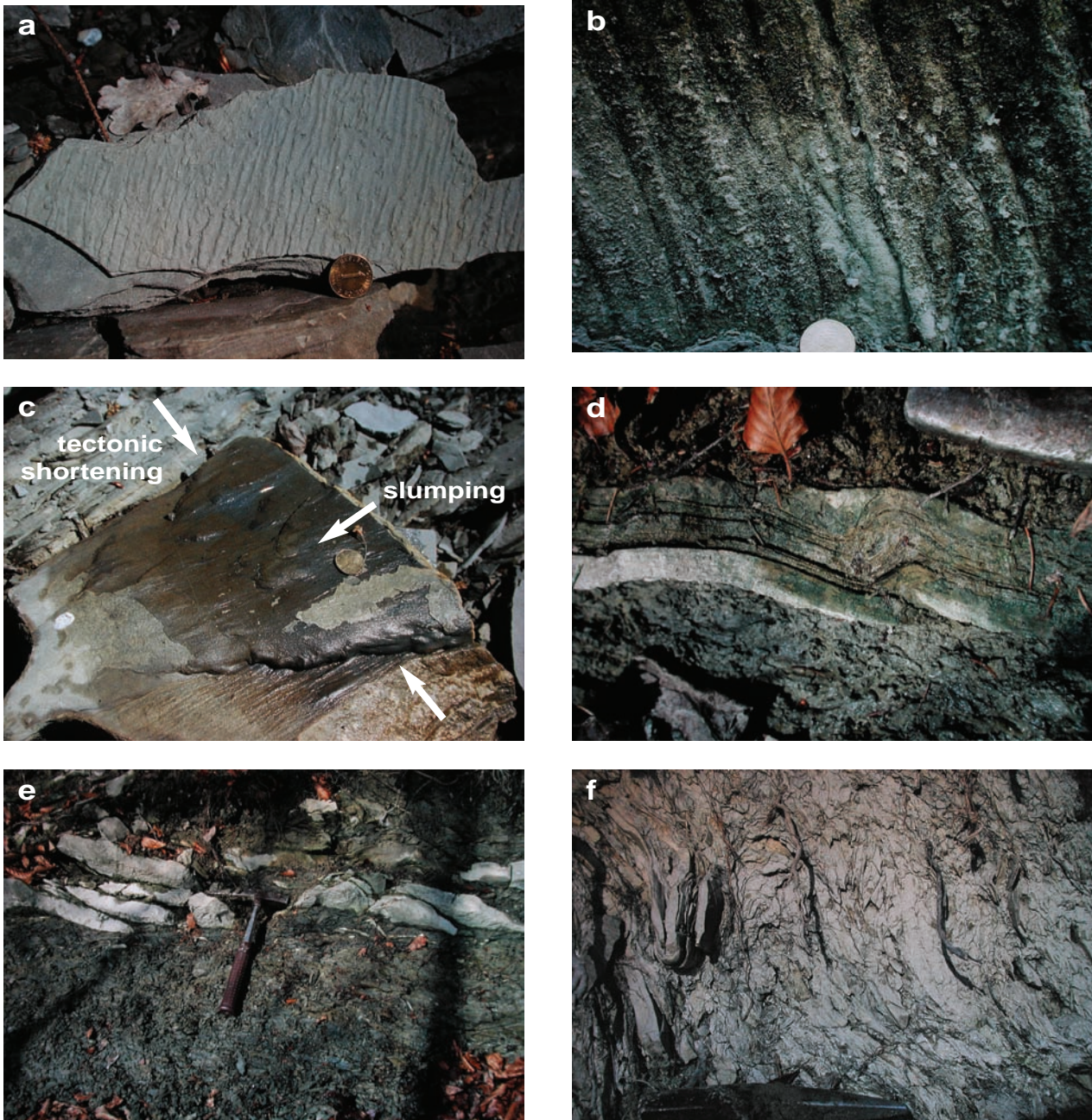
Fig. 13: Deformational structures in the Unterangerberg Fm. of the Unterangerberg. a) to e) illustrate progressive deformation by increasing bed-parallel shortening. a) incipient shortening leads to „crenulation“ of the siltstone-marl-interface at the base of a siltstone bed. b) cusate-lobate structure at the base of a sandstone bed. c) interaction of slumping and tectonic shortening at base of sandstone bed, both overprinting flute casts. d) formation of small scale blind thrusts above ramps, preserving a flat bed top. e) stacking of sandstone beds. f) shear zones with penetrative deformation.
