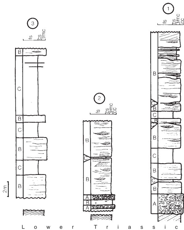
Fig. 5: Type section (1) of the Lengerergraben Mb. in the Schuhrergraben valley (stop 2). Sections 2 (Lengerergraben valley) and 3 ("Burg") illustrate the lateral facies changes in transport direction. A, B, C refer to the facies associations of STINGL & KROIS (1991).
