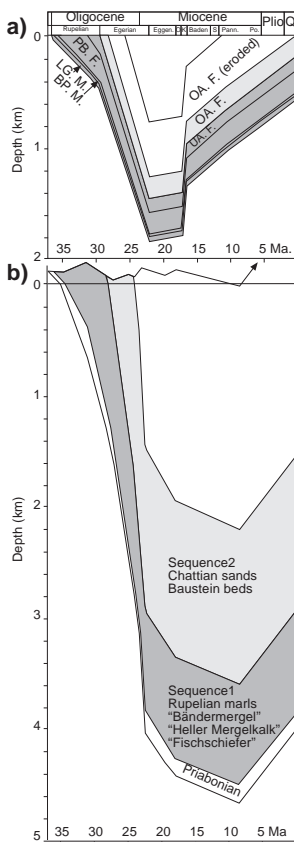
Fig. 20: a) Subsidence curve for the Oligocene in the Lower Inn Valley redrawn from Ortner & Sachsenhofer (1996). Timescale after Steininger et al. (1988/89) for Oligocene sediments and Steininger et al. (1990) for Miocene sediments. b) Subsidence curve for a well SSE of Munich in the Molasse basin simplified from Zweigel et al. (1998). Absolute ages taken from Harland et al. (1990) and Steininger et al. (1985). Minor differences between the curves due to differences in time scales. Abbreviations: BP. M. = Bergpeterl Mb., LG. M. = Lengerergraben Mb., PB. F. = Paisslberg Fm., UA. F. = Unterangerberg Fm., OA. F. = Oberangerberg Fm.
