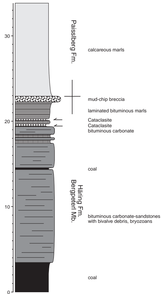
Fig. 6: Type section of the Bergpeterl Mb. in the Juliuschacht in the Bergpeterl quarry at stop 4.
