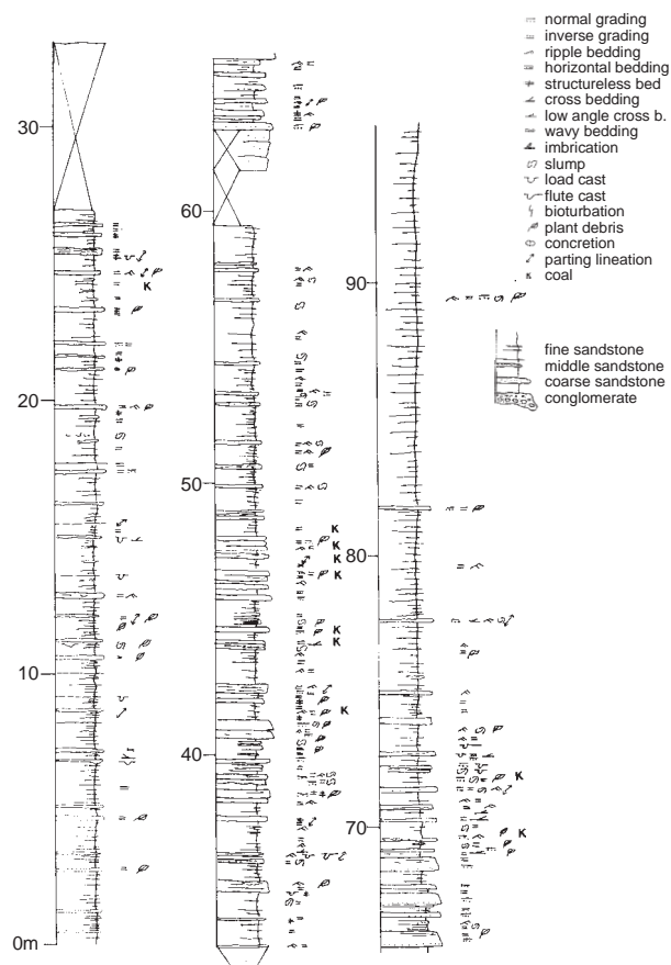
Fig. 11: Section Angath: Type section of the Unterangerberg Fm. at step 7.
