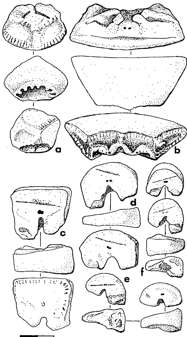
Fig. 3: Chelocrinus carnalli BEYRICH, 1856. Diplopora Dolomite, Piekary Śląskie. a Basal, from distal, aboral, lateral (top to bottom); GIUS-7-59/29. b Radial, from distal, aboral, proximal (top to bottom); GIUS-7-59/30. c Proximal tertibrachial with synostosomal proximal and muscular distal face; GIUS-7-59/31. d Tertibrachial with two muscular faces; GIUS-7-59/32. e Tertibrachial from middle to distal arm with a muscular and a synostosomal face; GIUS-7-59/33. f Tertibrachial from middle to distal arm with two muscular faces; GIUS-7-59/34. Scale 2 mm.
