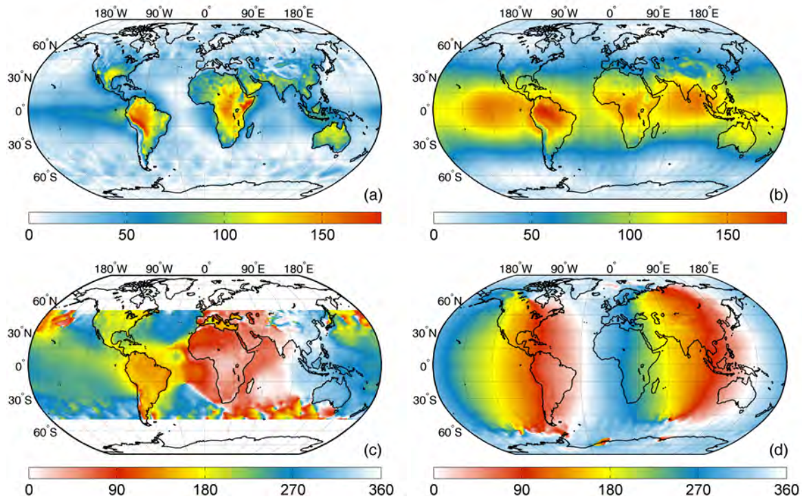
Figure 4.1: Diurnal (a) and semi-diurnal (b) surface pressure amplitudes [Pa], and the corresponding diurnal (c) and semi-diurnal (d) Greenwich phase lags [deg] as deduced from 3-hourly ECMWF pressure fields for the year 2011.
