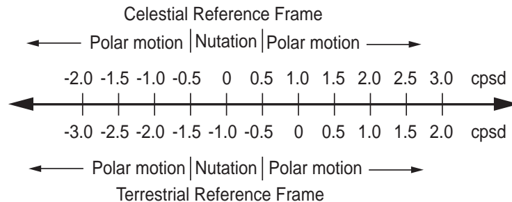
Figure 2.1: Relationship between the frequency of some motion as viewed from the celestial reference frame (top half of figure) and the corresponding frequency of the same motion as observed from the terrestrial reference frame (bottom half) (Gross, 2007; Schindelegger et al. , 2013b).
