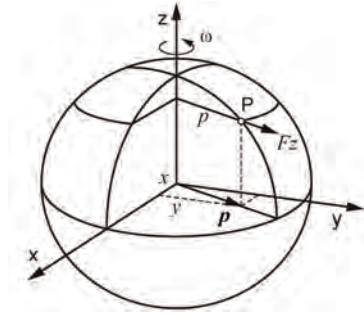
Figure 2.1: Centrifugal Force
