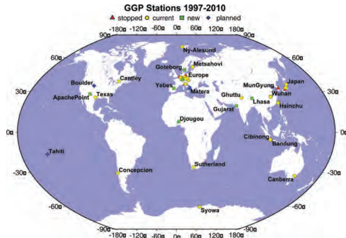
Figure 2.9: Network of the GPP, status of 2010, source: GGP project homepage http://www.eas.slu.edu/GGP/ggphome.html
