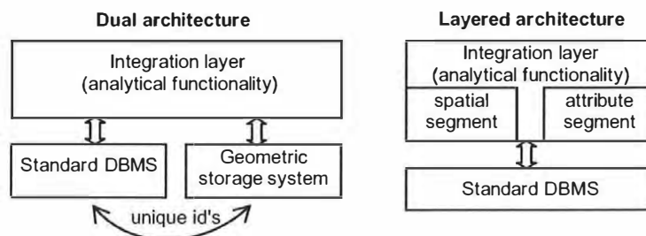
Figure 1: Early spatial data management systems architectures
