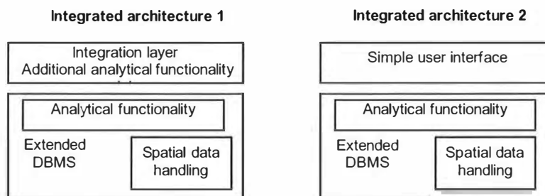
Figure 2: Contemporary system architectures
