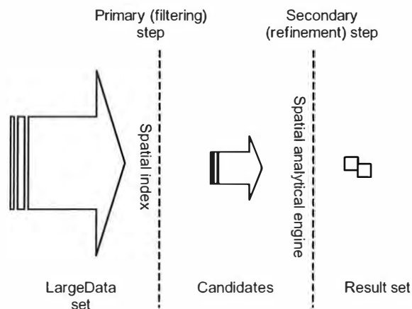
Figure 3: Spatial query processing
