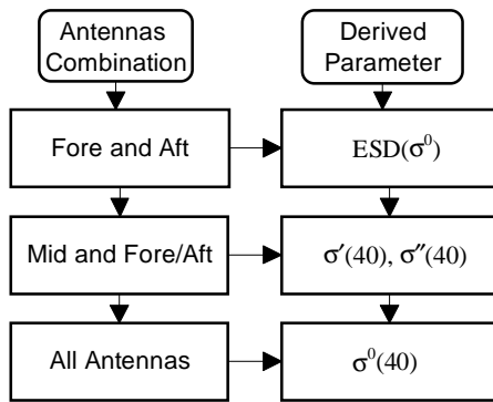
Figure 6-2: Flow chart of processing steps for the analysis of ERS Scatterometer data. In the processing four parameters are obtained: The estimated standard deviation of \sigma^0 , ESD(\sigma^0) , the slope \sigma'(40) and the curvature \sigma''(40) , and the normalised backscattering coefficient \sigma^0(40) .
