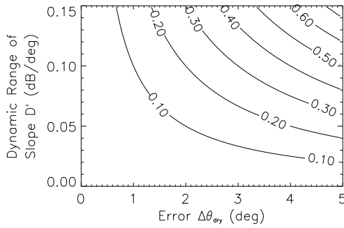
Figure 7-4: Contour plot of the maximum error of the backscattering coefficient of a dry soil, \text{Max}(\Delta\sigma_{dry}^0) in dB, in dependence on the dynamic range of the slope D' and the deviation of the estimated \theta_{dry} value from its real value, denoted by \Delta\theta_{dry} .
