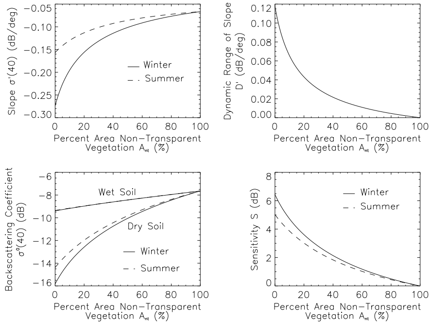
Figure 7-10: Simulated dependence of the slope \sigma'(40) , dynamic range of slope D' , backscattering coefficient \sigma^0(40) , and sensitivity S on the percentage area occupied by non-transparent vegetation A_{nt} using the model given in Table 5-1.
