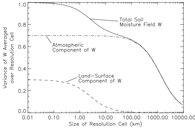
Figure 5-4: Reduction of the variance of the soil moisture field W according to Equation (5.14). Assumed values are \eta = 0.3 , L_s = 1 km, and L_a = 500 km.
