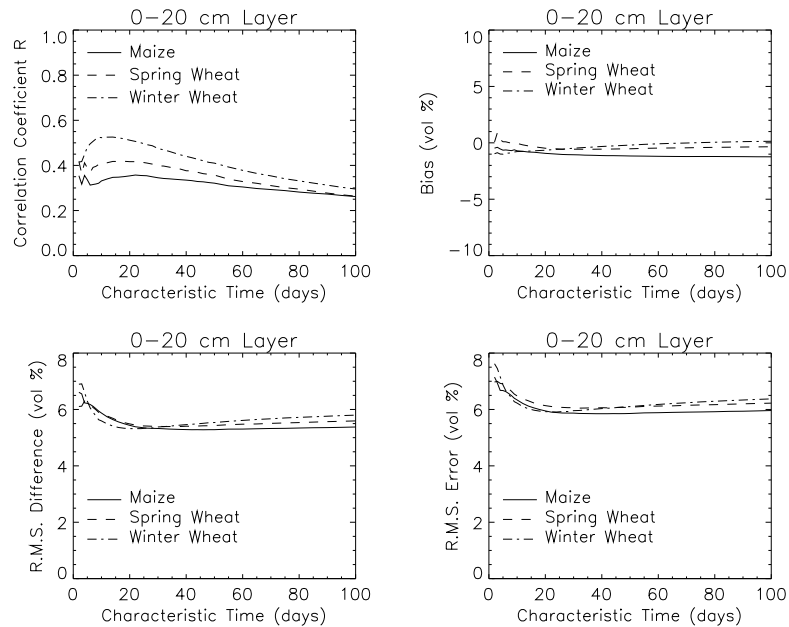
Figure 9-14: Correlation coefficient, bias, r.m.s. difference, and r.m.s. error versus the characteristic time length T for the 0-20 cm layer. The curves represent the mean values for 70 maize, 70 spring wheat, and 71 winter wheat fields.
