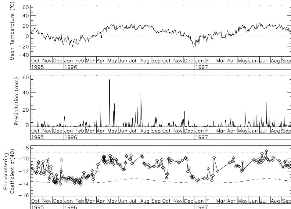
Figure 8-1: Time series of mean temperature, precipitation and \sigma^0(40) for the station Sarny (26.62°E, 51.35°N) for the period October 1995 to September 1997. In the bottom figure the backscattering coefficient of a dry and wet surface, \sigma^0_{dry}(40,t) and \sigma^0_{wet}(40) are indicated by dashed lines.
