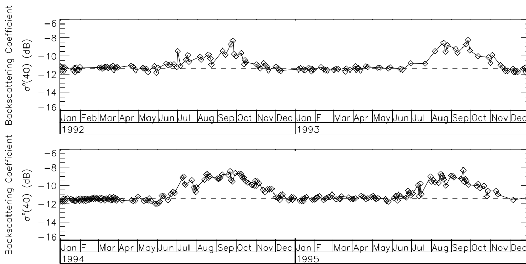
Figure 6-12: Time series of normalised backscattering coefficient \sigma^0(40) for a region in western Mali ( 11.8^\circ\text{W} , 13.6^\circ\text{N} ). The dotted line shows the mean value of \sigma^0(40) during the dry season.
