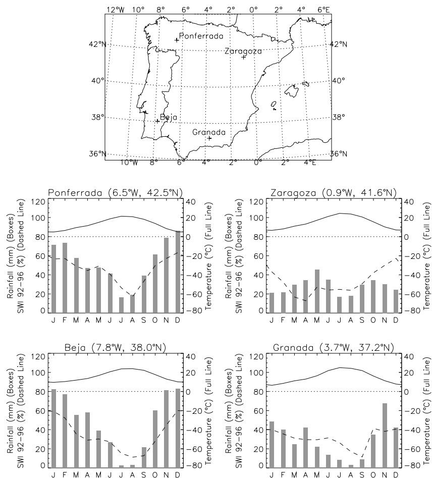
Figure 10-2: Climographs for four stations at the Iberian Peninsula. Also shown are the mean monthly SWI values from the years 1992-1996.
