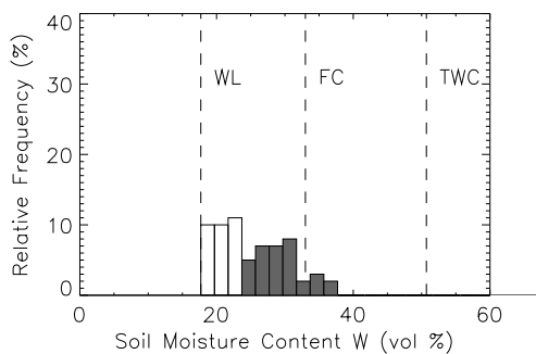
Figure 9-5: Histogram of soil moisture content W in % of the 0-100 cm layer at the winter wheat field at the station Belovodsk (39.58°E, 49.21°N). The field has a chernozem soil with a heavy loamy texture. The wilting level WL , field capacity FC , and total water capacity TWC are indicated by the dashed lines.
