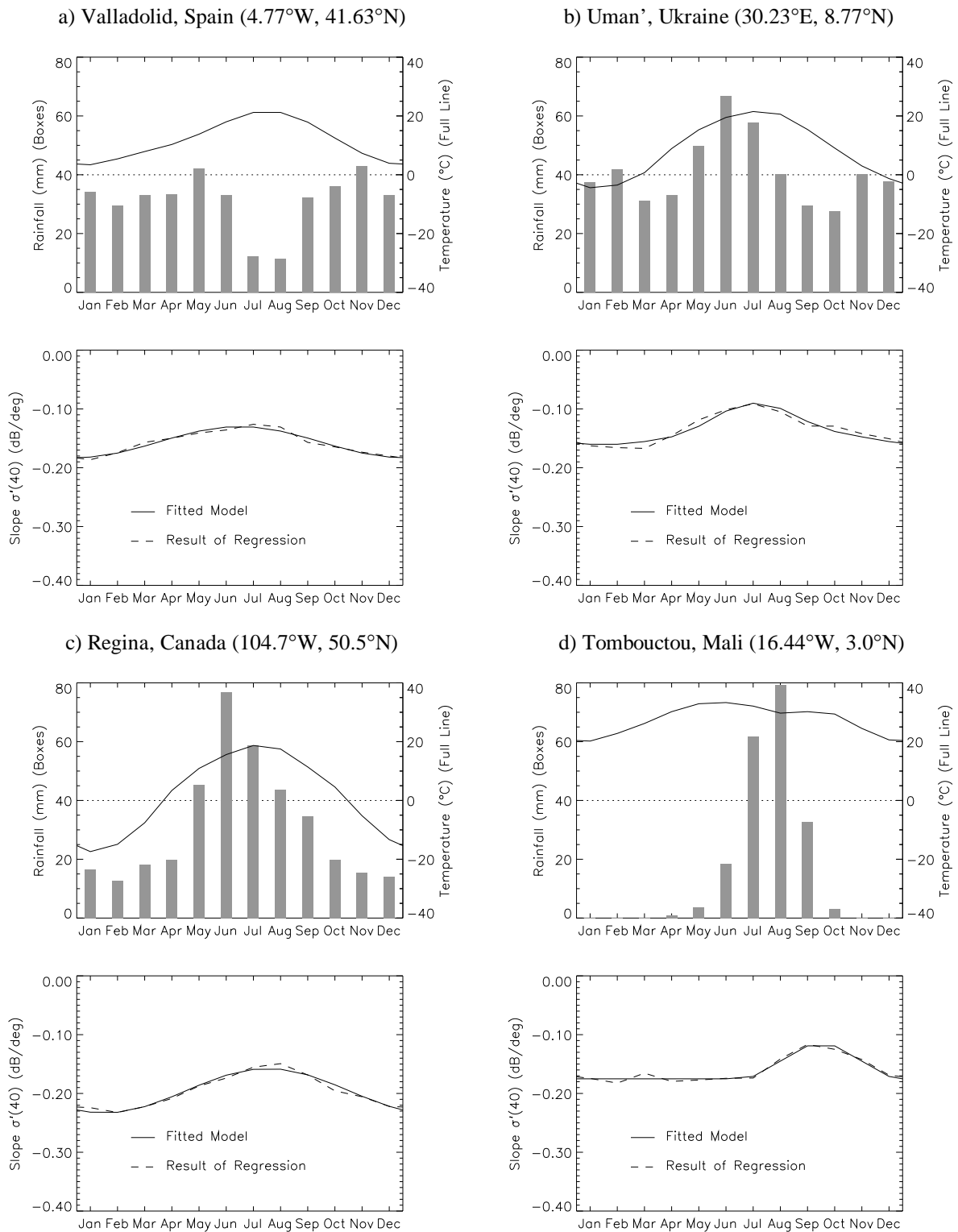
Figure 7-1: Climographs and seasonal variation of the slope \sigma'(40) for four sites in a) Spain, b) Ukraine, c) Canada, and d) Mali.
