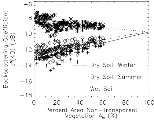
Figure 7-8: Scatter plot of the backscattering coefficient, \sigma^0(40) , versus the percentage area occupied by non-transparent vegetation types, A_{nt} . \sigma^0(40) values for dry and wet conditions are distinguished. For wet conditions \sigma^0(40) is very stable and indicated by the symbol * . For dry conditions \sigma^0(40) is somewhat higher in summer (symbol \diamond ) than in winter (symbol + ).
