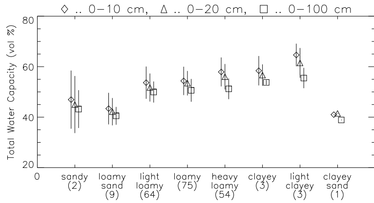
Figure 9-3: Same as Figure 9-1, but for the total water capacity TWC.
