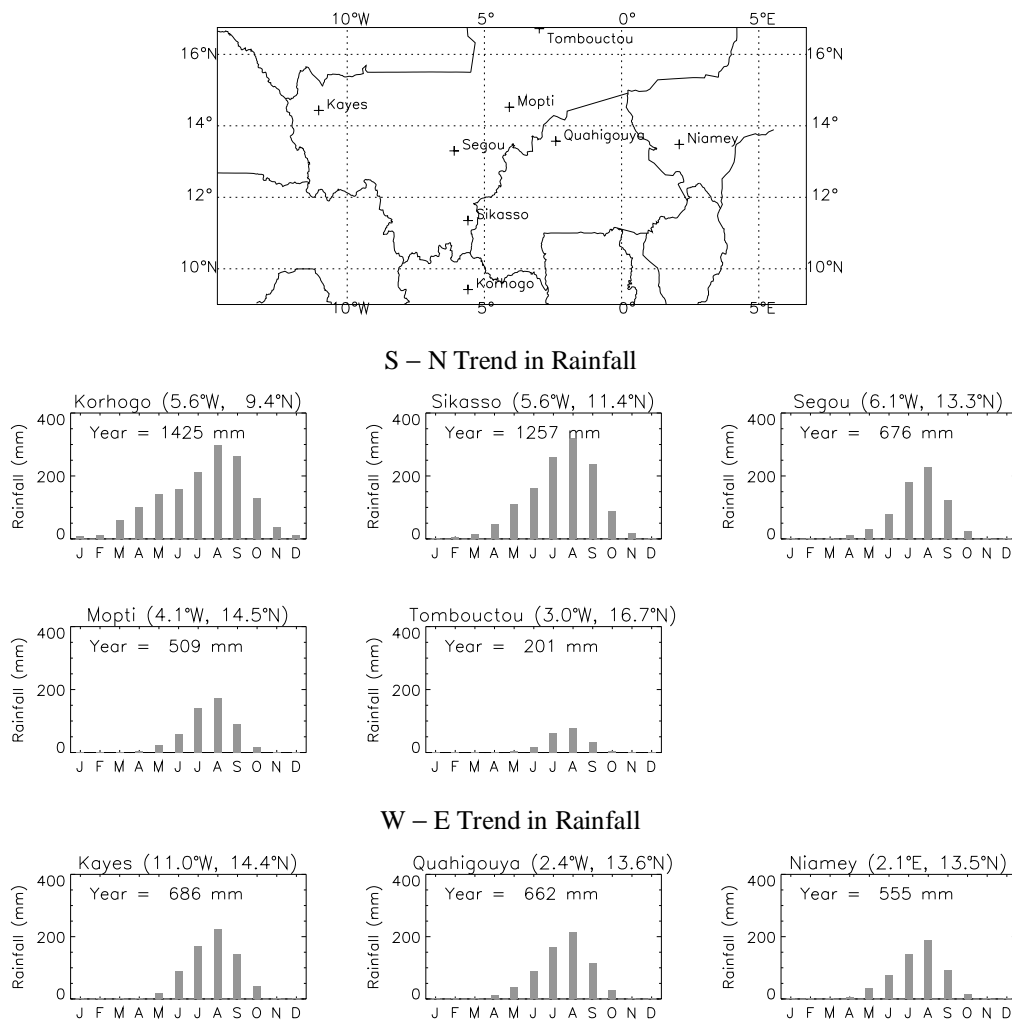
Figure 10-1: Average monthly rainfall for eight stations in the region 13°W-5°E and 9°N-16.5°N.
