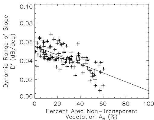
Figure 7-7: Scatter plot of the dynamic range of the slope, D' , versus the percentage area occupied by non-transparent vegetation types, A_{nt} .
