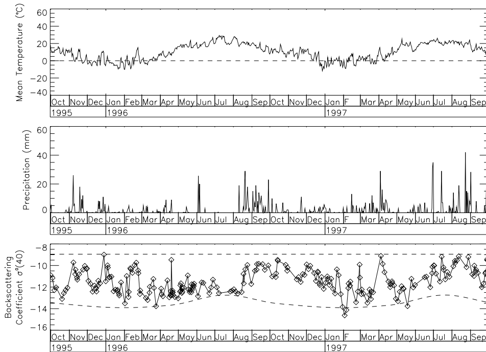
Figure 8-2: Same as Figure 8-1 but for the station Simferopol (33.98°E, 45.02°N).
