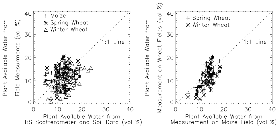
Figure 9-13: Scatter plots of plant available water PAW in % from ERS Scatterometer and field measurements for the station Prikolotnoye (37.4°E, 50.1°N). See caption of Figure 9-12.
