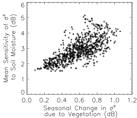
Figure 7-5: Soil moisture versus seasonal vegetation cover effects on the backscattering coefficient \sigma^0 based on the data set from the Iberian Peninsula.
