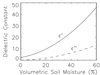
Figure 4-2: Dielectric constant \epsilon of a loamy soil versus the volumetric soil moisture content in %.
