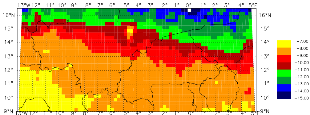
Colour Figure 5: Spatial variation of \sigma_{wet}^0(40) in dB over southern Mali and Burkina Faso derived from ERS Scatterometer data acquired during the period from September 1991 to January 1998.
