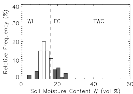
Figure 9-6: Histogram of soil moisture content W in % of the 0-100 cm layer at the winter wheat field at the station Sarny (26.65°E, 51.33°N). The field has a dark grey podzolic soil with a loamy sand texture. The wilting level WL , field capacity FC , and total water capacity TWC are indicated by the dashed lines.
