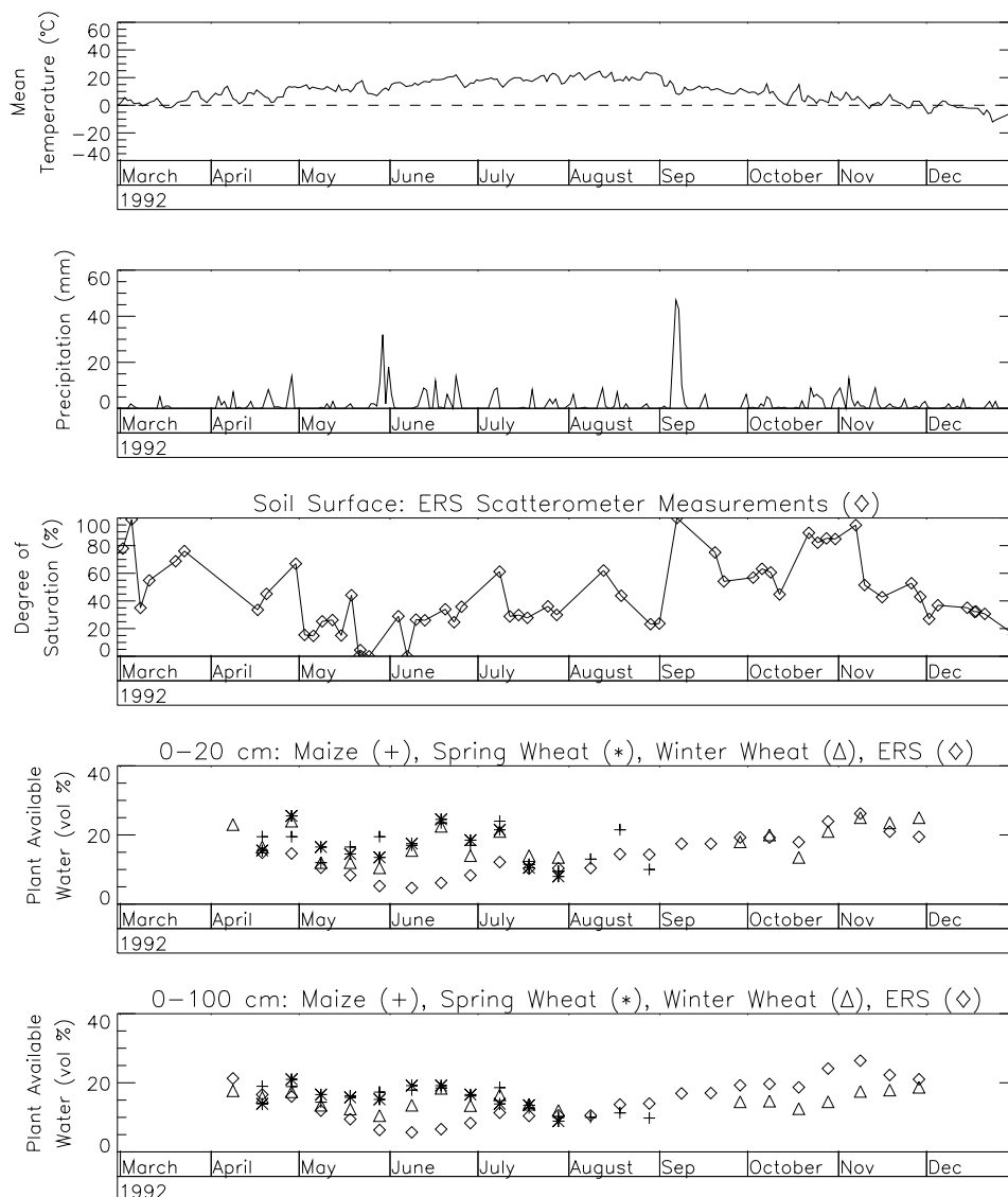
Figure 9-10: Meteorological observations, field measurements of soil moisture, and remotely sensed wetness values for Ternopol (25.6°E, 49.6°N) for the year 1992. The third diagram from the top shows ERS Scatterometer retrieved surface moisture m_s . The two diagrams on the bottom show plant available water content in % for the 0-20 cm and 0-100 cm layers measured on maize (cross), spring wheat (asterix), winter wheat (triangle) fields and the remotely sensed soil wetness values (diamond) according to Equation (9.7).
