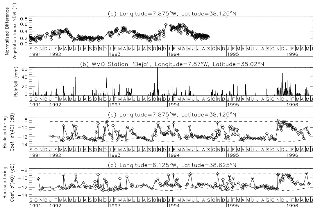
Figure 7-2: Temporal evolution of the NDVI, rainfall observations, and the backscattering coefficient, \sigma^0(40) over an agricultural region around Beja in southern Portugal. (a) Daily NDVI values degraded to match the resolution of the ERS Scatterometer. (b) Rainfall recorded at the synoptic station “Beja”. (c) \sigma^0(40) time series over Beja. The dotted lines show the backscattering coefficient for dry soil conditions, \sigma_{dry}^0(40,t) , and the backscattering coefficient for wet soil conditions, \sigma_{wet}^0(40) . (d) \sigma^0(40) series over a region about 150 km east of Beja. The dotted lines represent \sigma_{dry}^0(40,t) and \sigma_{wet}^0(40) .
