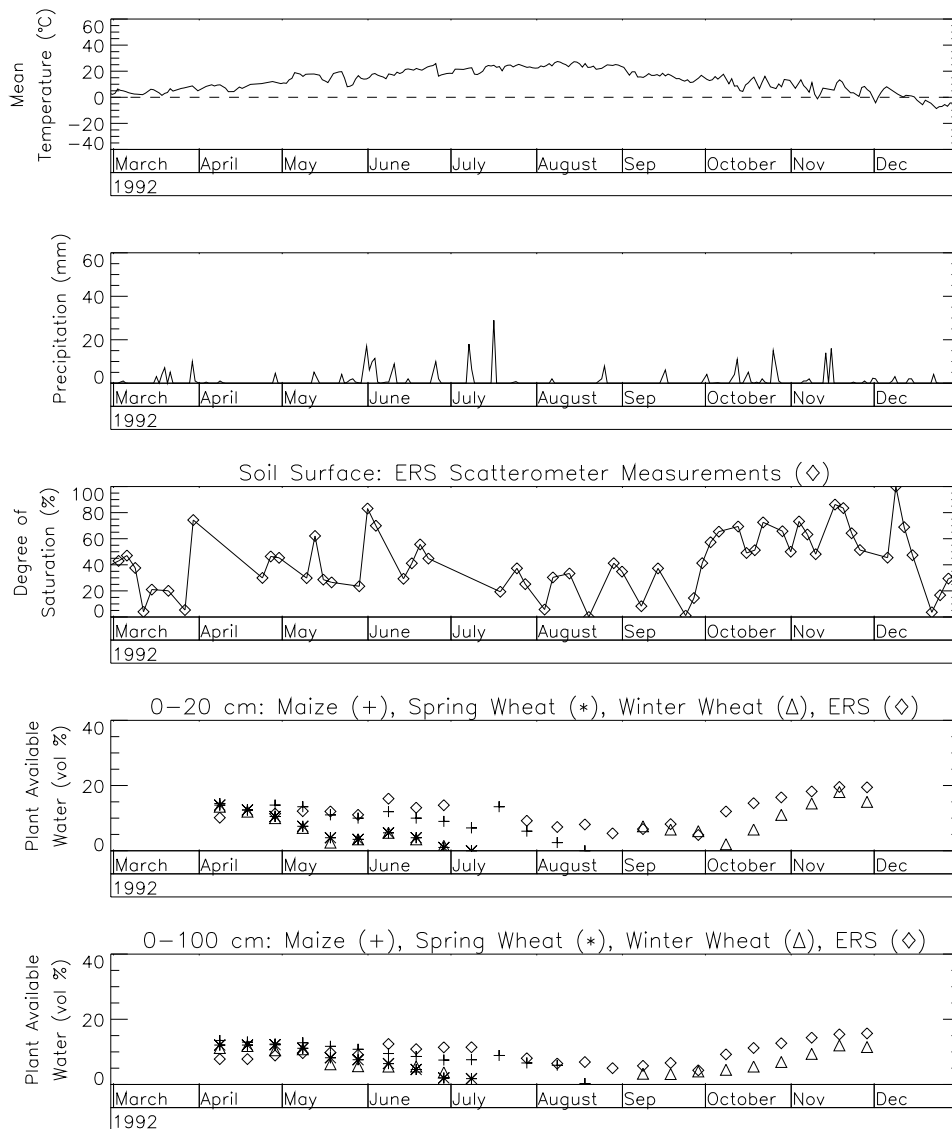
Figure 9-9: Meteorological observations, field measurements of soil moisture, and remotely sensed wetness values for Odessa (36.67°E, 46.47°N) for the year 1992. The third diagram from the top shows ERS Scatterometer retrieved surface moisture m_s . The two diagrams on the bottom show plant available water content in % for the 0-20 cm and 0-100 cm layers measured on maize (cross), spring wheat (asterisk), winter wheat (triangle) fields and the remotely sensed soil wetness values (diamond) according to Equation (9.7).
