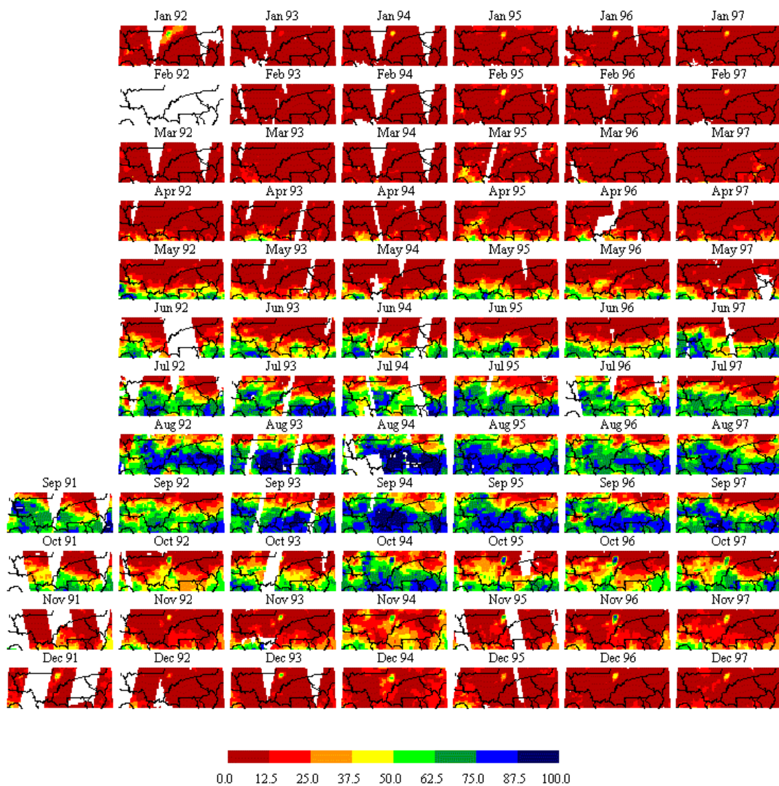
Colour Figure 10: Monthly SWI images of southern Mali and Burkina Faso ( 13^{\circ}\text{W} - 5^{\circ}\text{E} , 9^{\circ}\text{N} - 16.5^{\circ}\text{N} ) for the period from September 1991 to December 1997.
