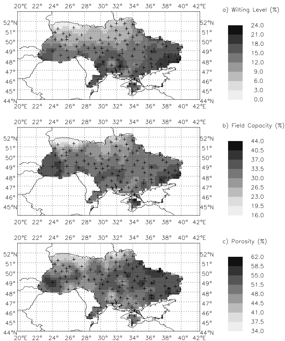
Figure 9-4: Soil constants for 0-100 cm soil layer interpolated to a 0.25° grid. The crosses indicate the location of the agrometeorological stations. a) Wilting level; b) Field capacity; c) Porosity or total water holding capacity. All constants are expressed in volumetric percent.
