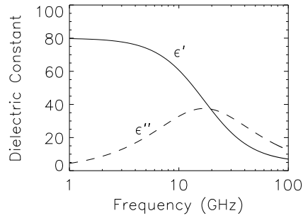
Figure 4-1: Dielectric constant \epsilon of pure water versus frequency at 20°C.
