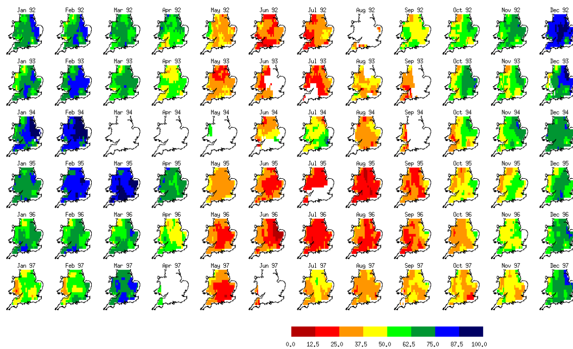
Colour Figure 13: Monthly SWI images for England and Wales for the period from January 1992 to December 1997.
