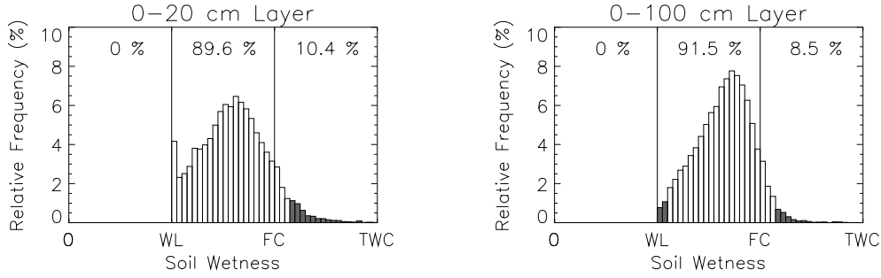
Figure 9-7: Histogram of soil moisture content in 0-20 cm layer (left side) and 0-100 cm layer (right side) based on measurements on 211 fields in the Ukraine. WL is the wilting level, FC the field capacity, and TWC the total water capacity
