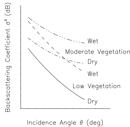
Figure 6-1: Characteristic angular dependence of the backscattering coefficient of vegetated surfaces for different moisture conditions. See also Figure 5-3.
