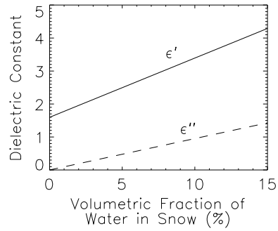
Figure 4-4: Dielectric constant \epsilon of snow versus the volume fraction of water in %.
