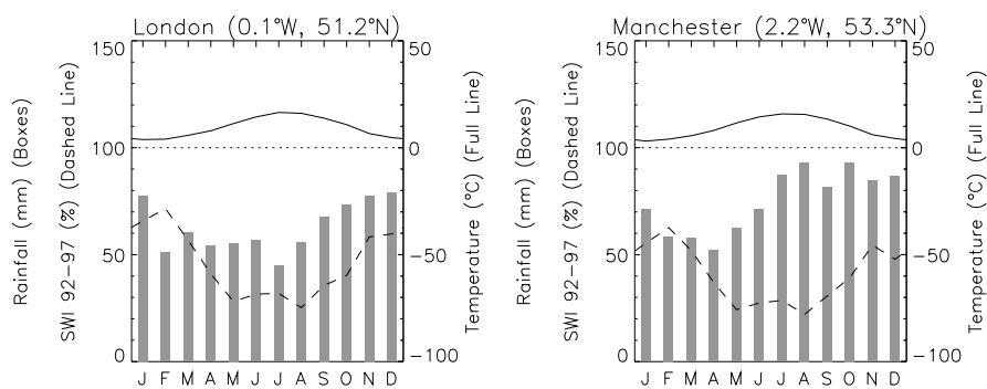
Figure 10-4: Climographs for London and Manchester. Also shown are the mean monthly SWI values from the years 1992 to 1997.
