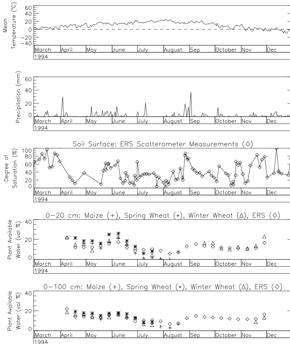
Figure 9-11: Meteorological observations, field measurements of soil moisture, and remotely sensed wetness values for Ternopol (25.6°E, 49.6°N) for the year 1994. The third diagram from the top shows ERS Scatterometer retrieved surface moisture m_s . The two diagrams on the bottom show plant available water content in % for the 0-20 cm and 0-100 cm layers measured on maize (cross), spring wheat (asterix), winter wheat (triangle) fields and the remotely sensed soil wetness values (diamond) according to Equation (9.7).
