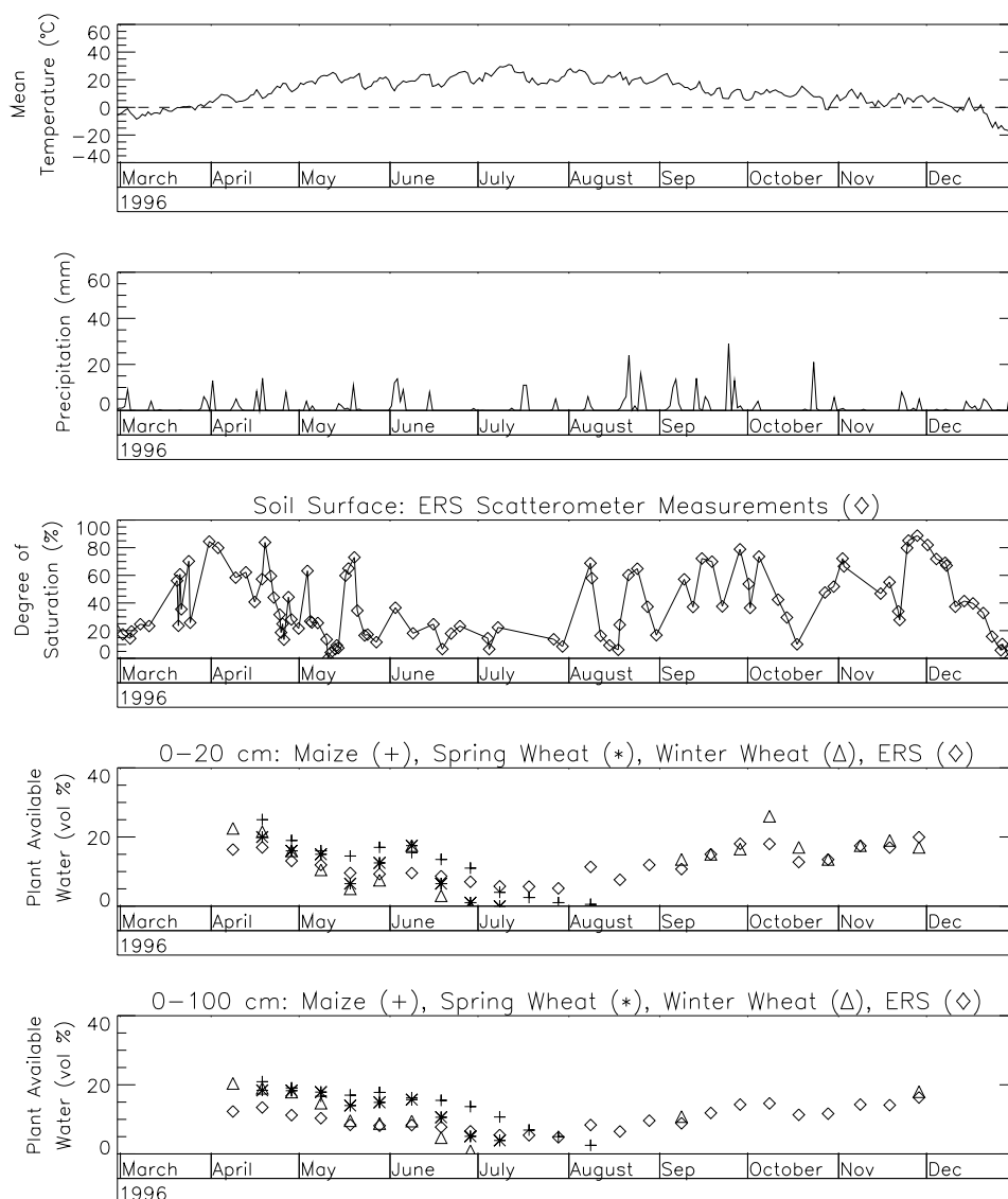
Figure 9-8: Meteorological observations, field measurements of soil moisture, and remotely sensed wetness values for Dnepropetrovsk (35.08°E, 48.37°N) for the year 1996. The third diagram from the top shows ERS Scatterometer retrieved surface moisture m_s . The two diagrams on the bottom show plant available water content in % for the 0-20 cm and 0-100 cm layers measured on maize (cross), spring wheat (asterix), winter wheat (triangle) fields and the remotely sensed soil wetness values (diamond) according to Equation (9.7).
