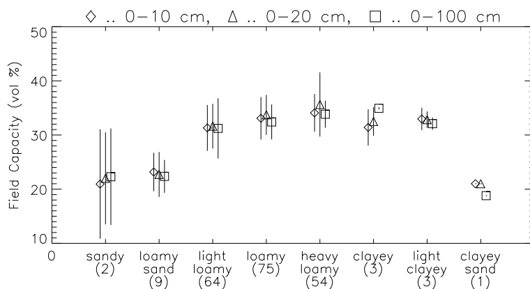
Figure 9-2: Same as Figure 9-1, but for the field capacity FC.
