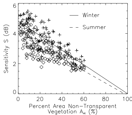
Figure 7-9: Scatter plot of the sensitivity S versus the percentage area occupied by non-transparent vegetation types, A_{nt} . Sensitivity values for t = \text{January 1} represent winter conditions (symbol + ) and for t = \text{July 1} summer conditions ( \diamond ).
