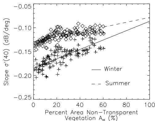
Figure 7-6: Scatter plot of the slope at 40^\circ , \sigma'(40) , versus the percentage area occupied by non-transparent vegetation types, A_{nt} . Slope values for t = \text{January 1} represent winter conditions and are indicated by a cross. Slope values for t = \text{July 1} represent summer conditions and are indicated by a diamond.
