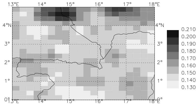
Figure 6-4: The estimated standard deviation of \sigma^0 , ESD(\sigma^0) , in dB over tropical forest in Africa (13°E-18°E, 0°N-5°N). The shown area partly covers Congo, Cameroon, Central African Republic, and Gabon. The map is based on ERS Scatterometer measurements from the year 1993.
