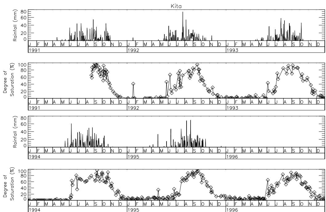
Figure 8-4: Rainfall and ERS Scatterometer retrieved m_s (degree of saturation) for Kita, Mali (9.28°W, 13.04°N) for the years 1991 to 1996. Rainfall data for the year 1996 are missing.
