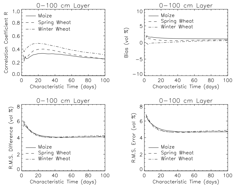
Figure 9-15: Same as Figure 9-14 but for 0-100 cm layer.
