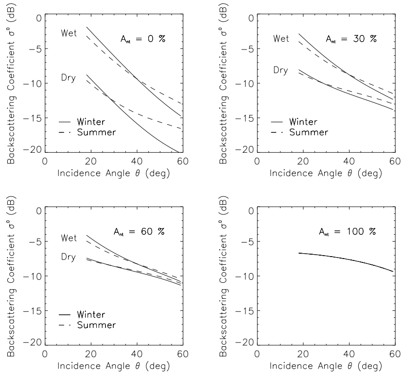
Figure 5-3: Simulated backscattering coefficient for increasing percentage area of non-transparent vegetation A_{nt} within one ERS Scatterometer pixel, and for dry/wet soil conditions and winter/summer conditions. The model and parameters used for the simulation are given in Table 5-1.
