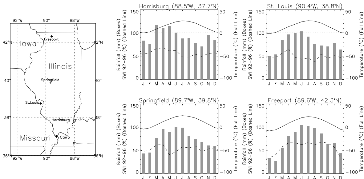
Figure 10-3: Climographs for four stations in Illinois, USA. Also shown are the mean monthly SWI values from the years 1992 to 1996.
