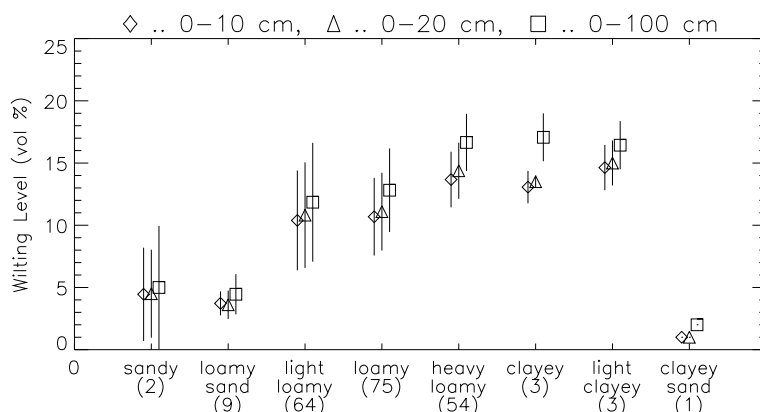
Figure 9-1: Wilting level, WL, in % for different soil textures and for three soil layers (0-10 cm, 0-20 cm, 0-100 cm) based on measurements on 211 fields in the Ukraine. The mean value and a bar representing the range mean value \pm standard deviation are shown. The numbers of field measurements on which these values are based are shown in brackets below the texture classes.
