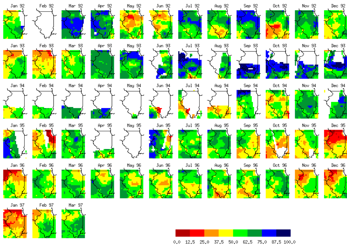
Colour Figure 12: Monthly SWI images for Illinois, USA (36°N-43°N, 87°W-92°W) for the period from January 1992 to March 1997.
