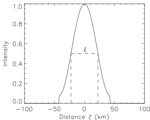
Figure 2-2: The Hamming window with a sidelength of 85 km. The dashed lines explain the definition of the spatial resolution l
