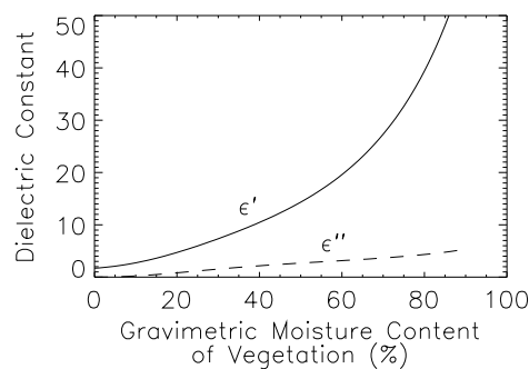
Figure 4-3: Dielectric constant \epsilon of vegetation versus the gravimetric soil moisture content in %.
