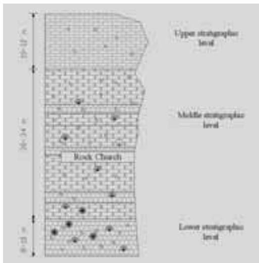
Figure 20 - Geological profile
