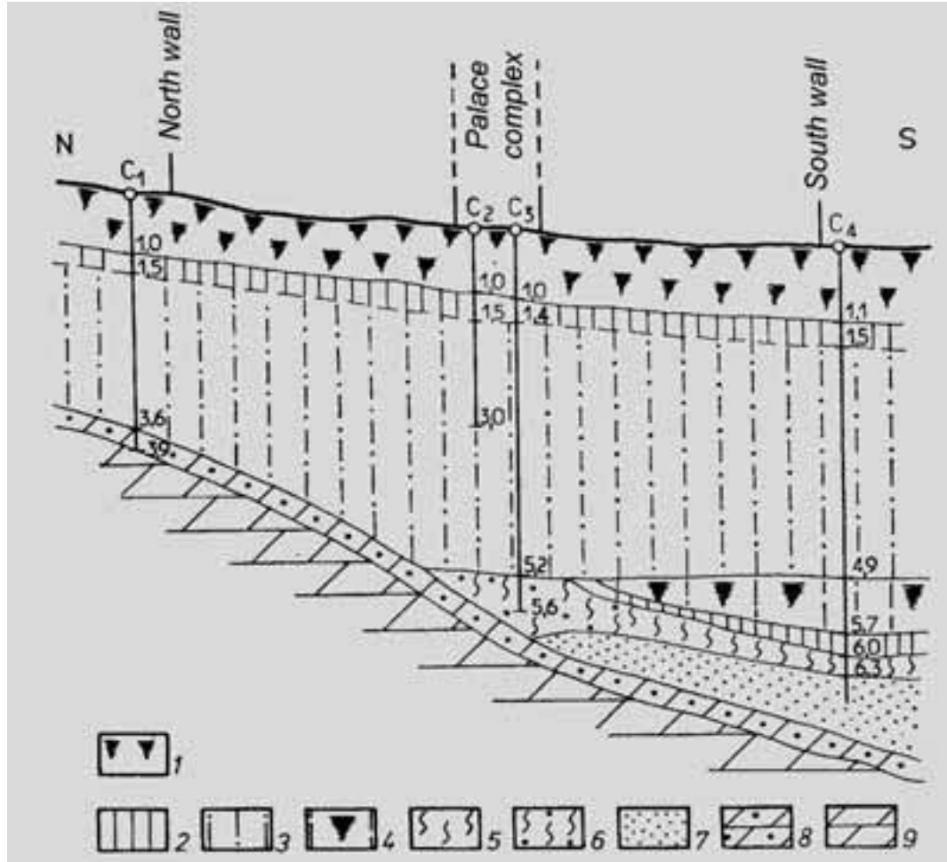
Figure 9 - Geological profile of Pliska (Evstatiev et al., 1983): 1-topsoil; 2-calcareous layer; 3-loess; 4-palaeosoil; 5-sandy-silty clay; 6-sandy-gravelly clay; 7-sand; 8-weathered marl; 9-marl
