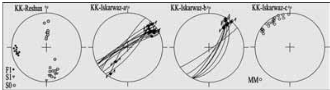
Figure 8.2. - Plot of mesoscopic structures measured in the Reshun Conglomerate and adjacent rock units.
