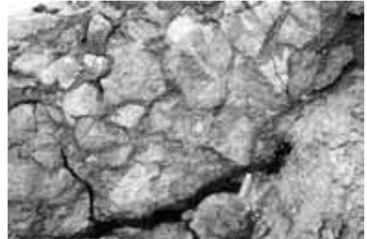
Figures 10 D1-2 - Col Rodella: arrival site of the cableway. Contact of the pillows breccias on the carbonate breccias of the Ladinian platform (Sciliar Dolomite Fm). Note the unconformity marked by dark crust (hard ground) along the irregular contact sealing the underlying dolomite breccias (Figure 10 D1). The structure of the underlying carbonate breccias is evidenced by the matrix septa (Figure 10 D2).
