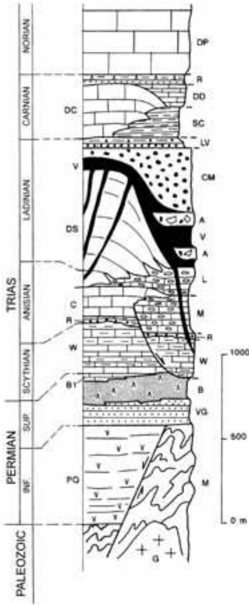
Figure 6 - Synthetic stratigraphy of the pre-Jurassic succession of the Western Dolomites. Letters: M, metamorphic rocks of the crystalline basement (Pre-Permian); G, Granodiorite intrusions (Early Permian); PQ, volcanics (quartz porphyry) (Early Permian); VG, Val Gardena sandstone Fm (Late Permian); B, B1, Bellerophon Fm (Late Permian): evaporitic (B) and shelf carbonate (B1) facies (late Permian); Werfen Fm (Early Triassic); R, Richthofen conglomerate Fm (Early Mid Triassic); C, Contrin Dolomite Fm (Anisian); M, Moena Fm (Anisian); L, Livinallongo Fm (Anisian-Ladinian); DS (PL), Sciliar Dolomite Fm (Ladinian carbonate Platform or buildup) (Anisian-Ladinian); V, volcanics (basalt) and sub-volcanics (basaltic dyke) (Late Ladinian); A, chaotic assemblage ("Agglomerate"); CM, Marmolada conglomerate Fm (Late Ladinian); LV, La Valle Fm (or Wengen Fm) (Late Ladinian); SC, San Cassiano Fm (Carnian); DC, Cassian Dolomite Fm (Carnico); DD, Dürrenstein Dolomite Fm (Carnico); Raiblian beds Fm (Carnico); DP, Dolomia Principale (Norico). From Castellarin et al., 1998a.
