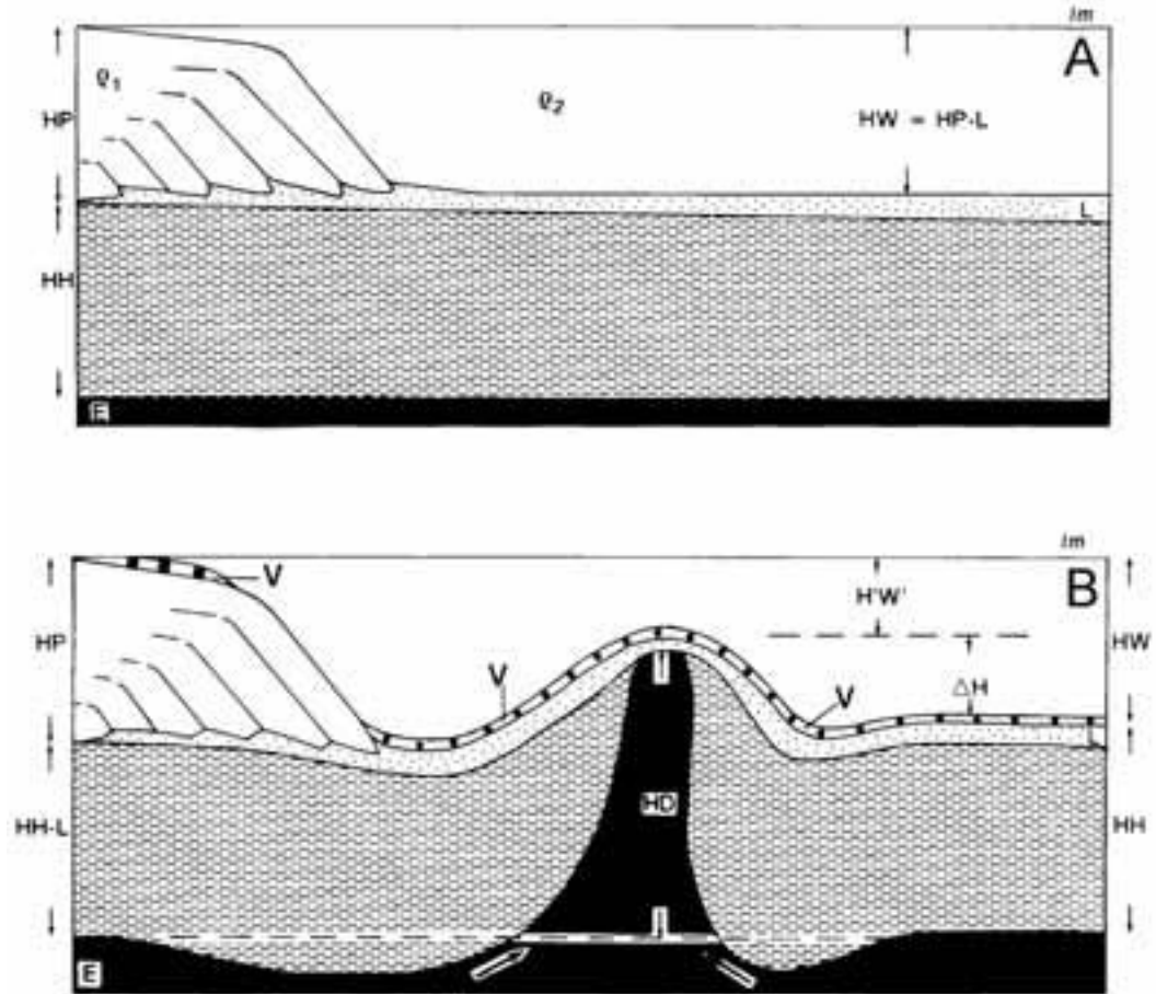
Figs.12 A, B - Relationships between Sciliar Dolomite buildup and the Livinallongo Fm basinal deposits predating the diapiric intrusion (12A). Simplified geometries of a diapiric anticline where the difference in overburden is provided by the difference in density of Sciliar Dolomite ( \rho_1 ) and sea water ( \rho_2 ) (12B). Letters: E, Permian evaporites; HH, stratigraphic units overlying the evaporites; HP, Sciliar carbonate platform succession (about 800m thick including volcanics); L, Livinallongo Fm (about 100 m thick including volcanics); V, volcanics (Figure 12 B); HW(= HP-L) depth of the basinal zone; average density of the Sciliar Dolomite (assumed value of some 2,5 gr/cm 3 ); density of sea water (assumed value of 1,035); HD, height of the diapiric structure (from evaporite source to top); H, height of the diapiric top (from the sea bottom); HH-L, interval of common units across the basin; overburden differential = (HP-L). \rho_1 - \rho_2 = 102,55 Bars (10,25 MPa). Modified from Castellarin et al., 1998b.
