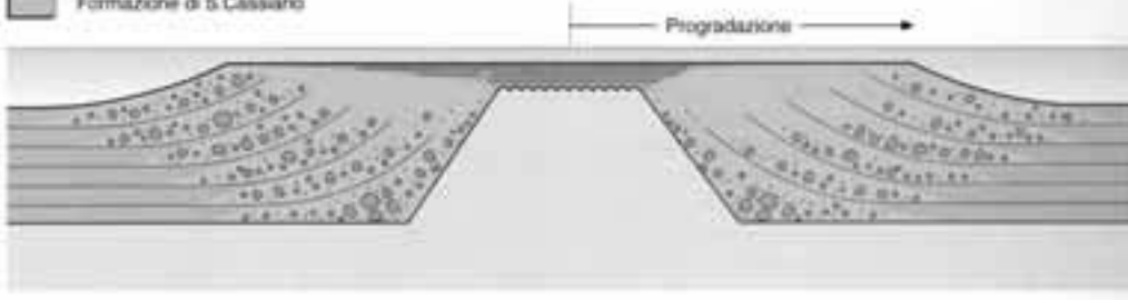
Figure 8 - Synthetic schemes illustrating different models controlling the relationships between carbonate shelf edifices during the mid Triassic time : in particular the Anisian-Ladinian buildups pre-dating the volcanic events and those (mostly Carnian) postdating the Volcanism. In the second case the progradation is strongly greater than aggradation due to the lower rate in subsidence. From Bosellini,1996
