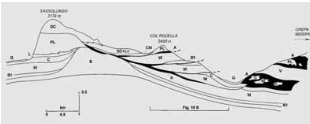
Figure 10 C - Geological section across the Col Rodella between the Sassolungo (Langberg) (to the N) and the Buffaure massif (to the S). The superposition of several Permian-Triassic slabs, previously referred to Mid Triassic or Neogene compressional duplication, are here related to gravitational Mid Triassic huge slides discharged from the S limb of a prominent diapiric anticline (modified from unpublished section by Eugenio Del Pero). Letters as in Figs. 6, 9, 10B.
