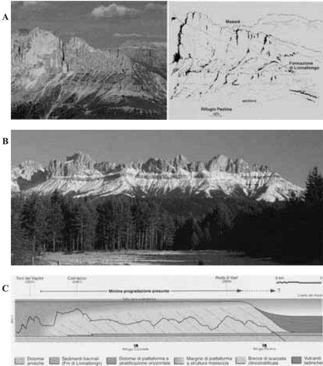
Figs. 7 A, B, C - Rosengarten (Catinaccio) W side: Roda di Vael and Masaré peaks: relationships between the Mid Triassic shelf carbonate (Sciliar Dolomite Fm) and the basinal coeval deposits (Livinallongo Fm). To be noted the clinoform thick beds of the the Sciliar Fm corresponding to the shelf slopes joining the tabular beds of the Livinallongo Fm in the basinal zone according to typical progradation geometries (Figure 7 A); panoramic view of the Rosengarten (Catinaccio) W side (Figure 7 B) and graphic synthetic reconstruction of the relationships between the different parts of the carbonate buildup and the basinal deposits documenting, in some 5 km, the minimal N to S progradation of the carbonate platform (Figure 7 C). In the same scheme (Figure 7 C) a reconstruction of the carbonate edifice zones missing, due to erosion, is also proposed. From Bosellini, 1996.
