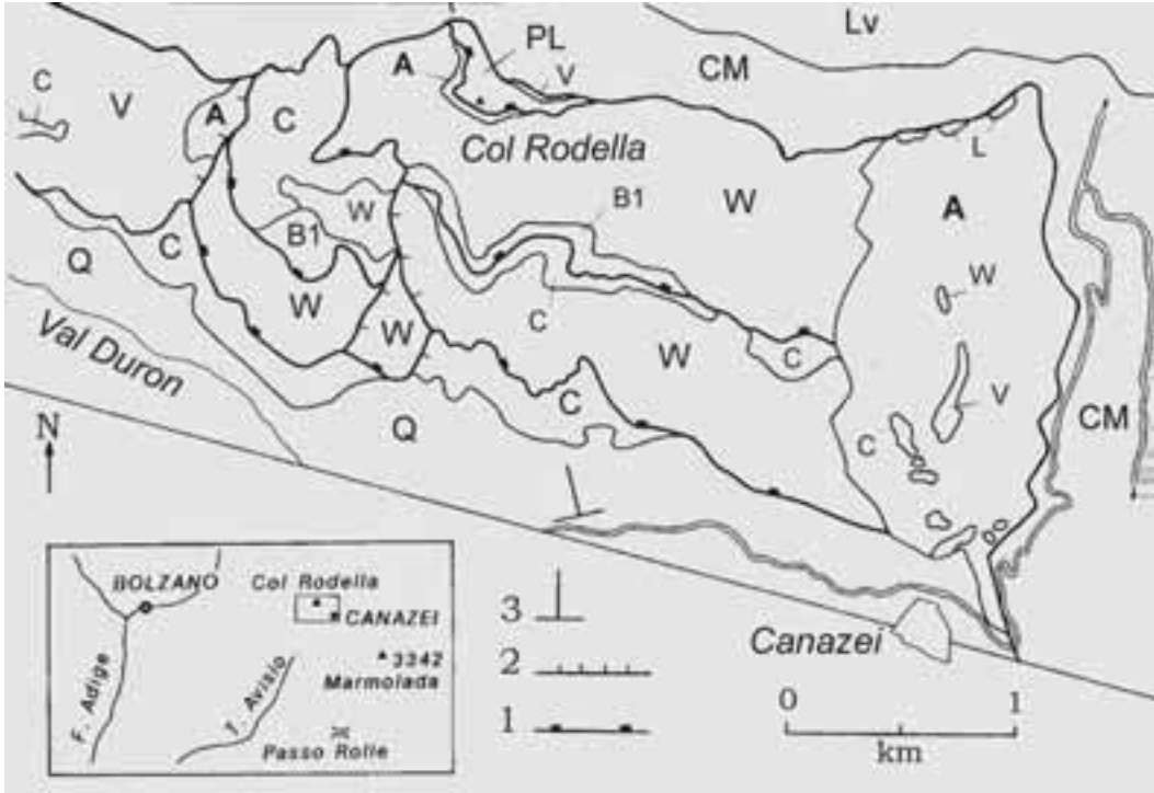
Figure 10 B - Very simplified geological map of the Col Rodella and surrounding zones (modified from unpublished map by Eugenio Del Pero). Letters as in Figs. 6,9; B1, Bellerophon Fm, carbonate shelf "badiota" facies; Lv, LaValle or Wengen Fm; Q, Quaternary cover. Numbers: 1, contact between superposed slab; 2, extensional fault; 3, trace of the geological section of Figure 10C (central part).
