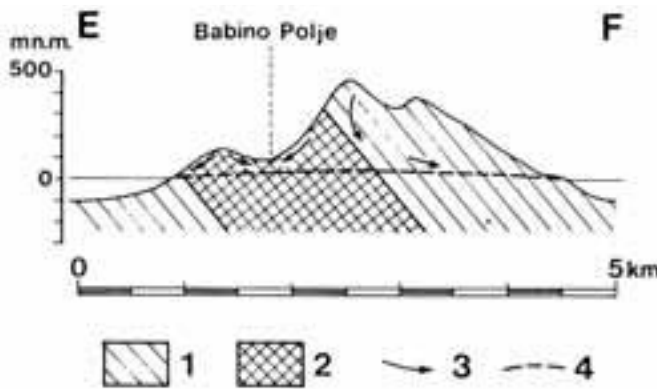
Figure 5.4 - Schematized hydrogeological profile of Mljet Island. Explanation: 1. Mostly limestones, 2. Dolomites, 3. Supposed directions of underground water-flow, 4. Supposed level of underground water.
