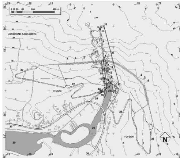
Figure 6.6 - Review sketch of the Ombla power plant facilities:
