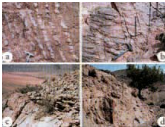
Figure 5a - Marly Rosso Ammonitico. Local facies in the Mellah. Aalenian-Lower Bajocian. Aïn Beïda , eastern slope of Djebel Mellah (Naâma wilaya).
