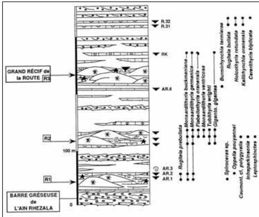
Stop 7b - Biostratigraphy and summarized log of the Upper Bajocian to Lower Bathonian .
