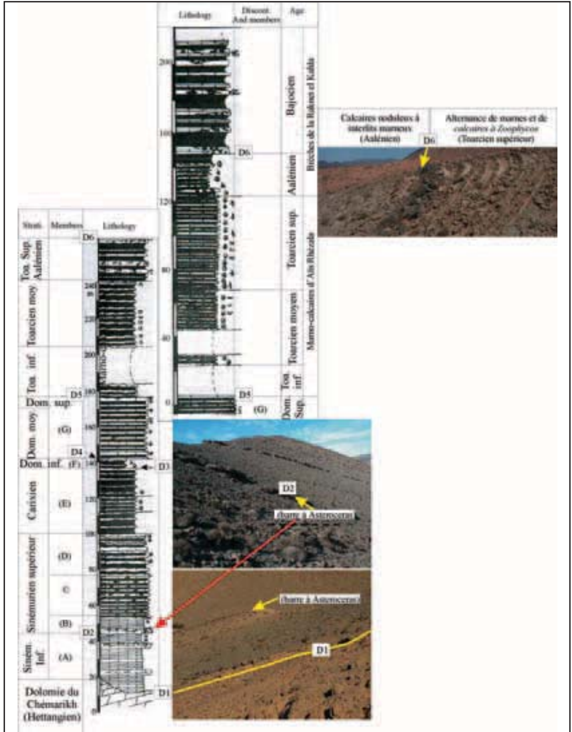
Figure 6 - Stratigraphic profiles of the Chemarikh (outcrop C/CK in the Ain Ouarka area)
