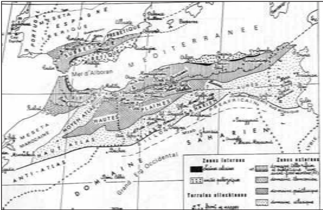
Figure 2 - Structural map of the western Mediterranean and the studied areas (Benest, 1985)
