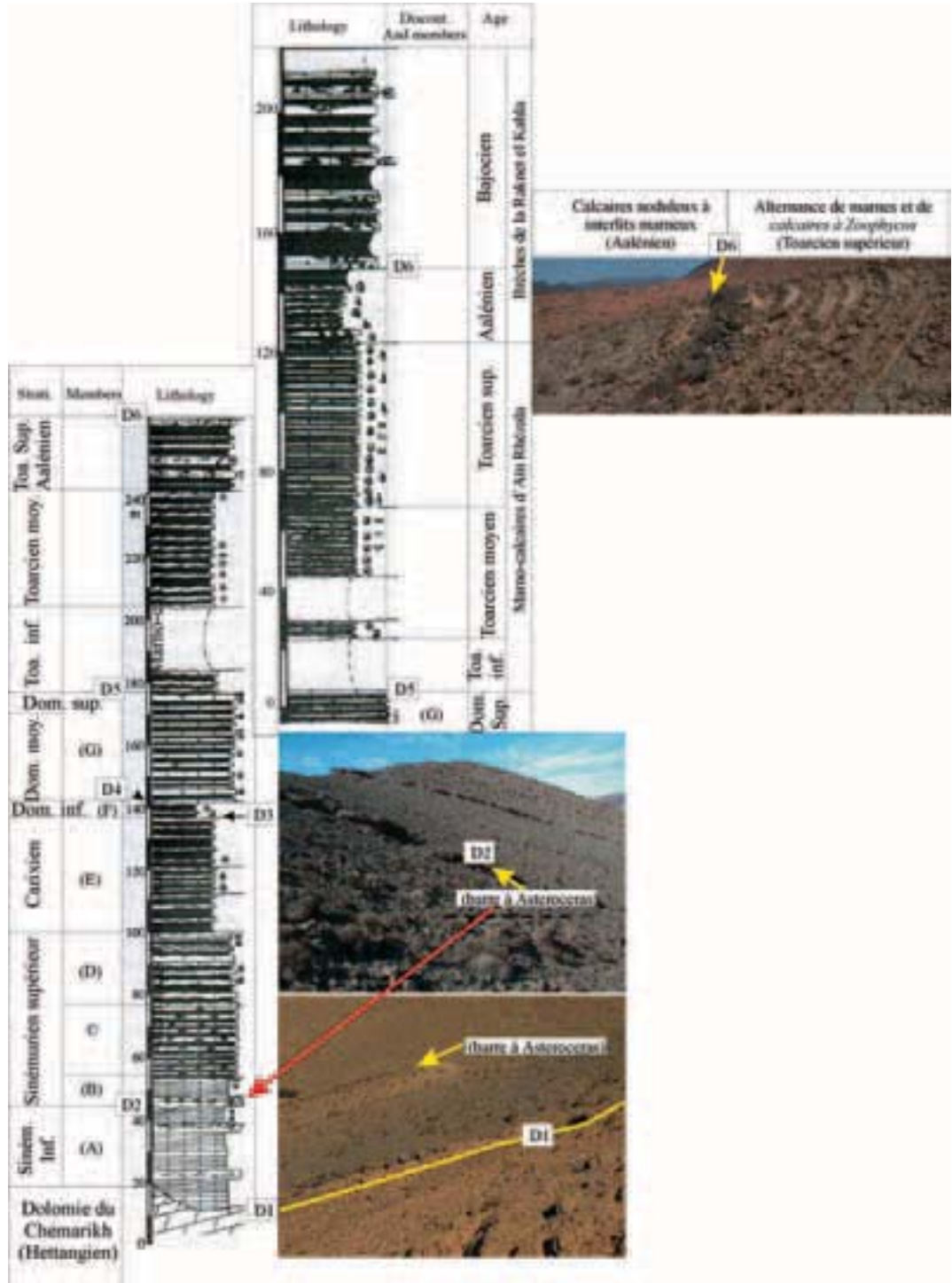
Stop 8 - Stratigraphic profiles of the Chemarikh (outcrop C/CK in the Ain Ouarka area)
