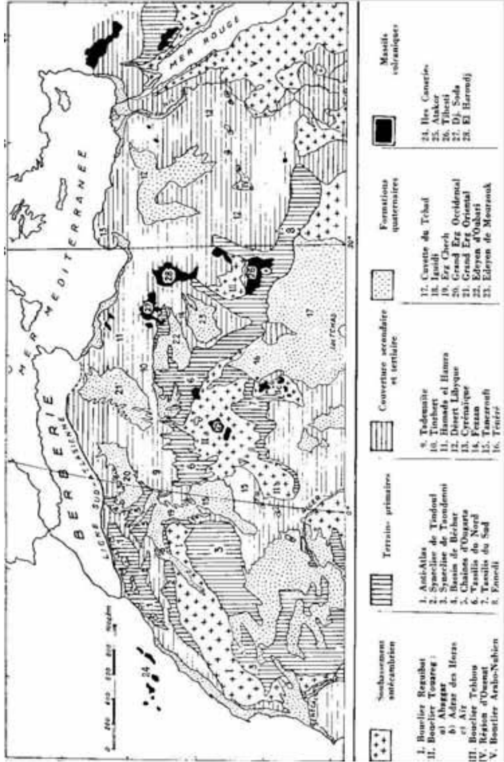
Figure 1 - The Maghreb system and its position on the northern margin of Africa (Menchikoff, 1947)
