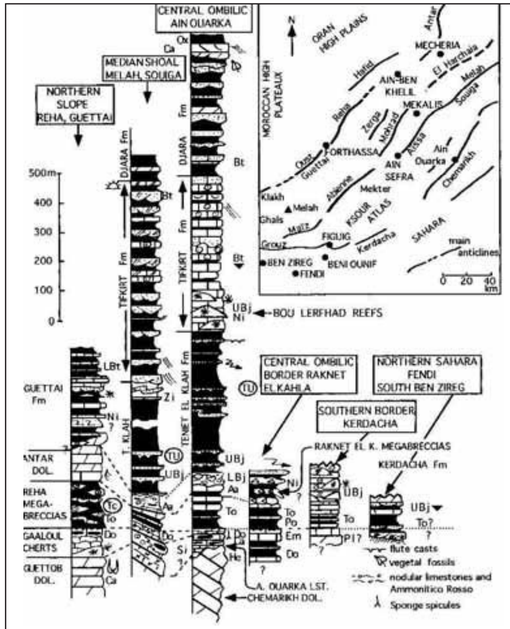
Figure 3 - Comparison of the stratigraphic profiles through the Saharian Atlas (Ksour mountains) from the northeastern marginal folds to the Sahara (South of Ben Zireg, between Bechar and Figuig). Each log is a synthesis of several measured sections. Abbreviations of stages, zones and facies symbols: He= Hettangian, Si = Sinemurian, Ca= Carixian, Do= Domerian, To= Toarcian, Aa= Aalenian, LBj= Lower Bajocien, UBj= Upper Bajocian, Bt= Bathonian, LBT= Lower Bathonian, PI= Planorbis, Em= Emaciatum, Po= Polymorphum, Ni= Niortense, Zi= Zizag, Tc= calciturbidites, TU= Quartzose turbidites. From Elmi et al., 1998.
