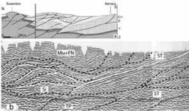
Figure 17 - (a) Geoseismic cross-section showing the subsurface structure at Rocca Busambra and Monte Barracù; same legend as in Figure 16. (b) Interpreted seismic image duplex deformation of the Sicanian Units (Si). Mu+FN: Numidian Flysch and Mufara Fm. ST: Oligo-Miocene cover. TP: Trapanese Units.
