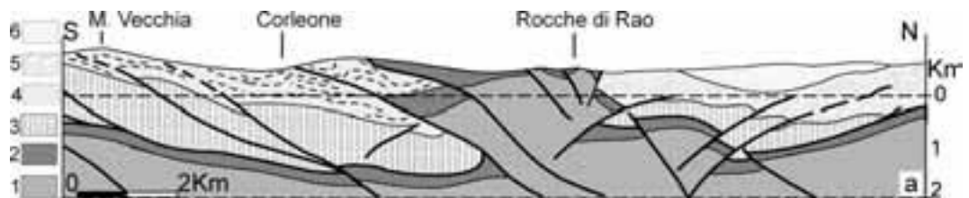
Figure 16 - Rocca Argenteria. Geoseismic profile (a) displaying the subsurface structural relationships between the Trapanese platform (1) terrigenous cover (2) outcropping in the Rocche di Rao ridge (shown in b) and the basinal Sicilian and Imerese Units (3,4). Numidian Flysch nappe (5) and molassic U. Miocene deposits (6).
