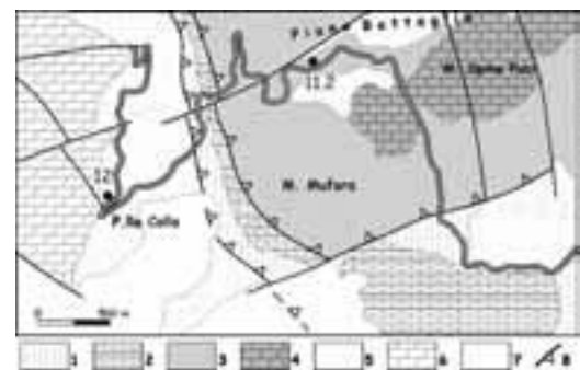
Figure 48 - Simplified geological map of the Portella Colla area. Marls and limestones (1), Mesozoic dolomites (2) (Quacella Unit). Triassic-Liassic (3) and Jurassic-Cretaceous platform carbonates (4) pertaining to the Panormide tectonic Unit. Numidian Flysch (5) and Imerese basinal carbonates (6) (Monte dei Cervi Unit), Debris (7). Mod. from Abate et alii (1982).
