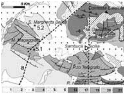
Figure 27 - Structural map of Monte Magaggiaro-Pizzo Telegrafo and traces of geoseismic sections. Same legend as in Figure 25.
