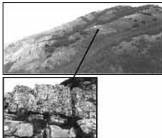
Figure 51 - Nipitalva Valley. Panoramic view of the Triassic-Lower Liassic Imerese Basin sequence.
