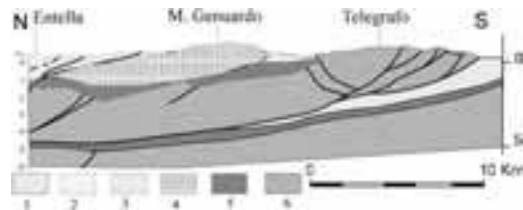
Figure 29 - Geoseismic section (b in Figure 27), showing the relationships between Monte Genuardo and Pizzo Telegrafo units. 1. Plio-Pleistocene deposits; 2. U. Miocene terrigenous and evaporitic deposits; 3. M. Miocene terrigenous cover of 4. Monte Genuardo carbonate succession; 5. M.-U. Miocene cover of 6. Trapanese-Saccense units.
