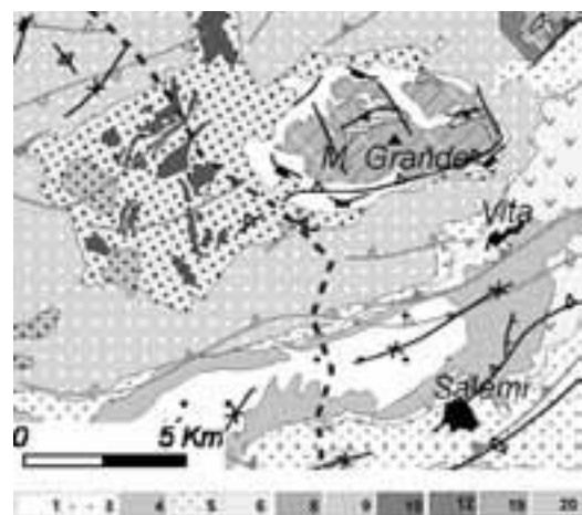
Figure 31 - A) Structural map of Montagna Grande area. The trace of seismic sections of Figure 33 is also shown.
