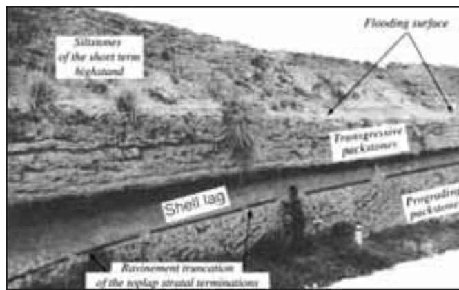
Figure 43 - Mulino del Barone. The Capodarso parasequences.
