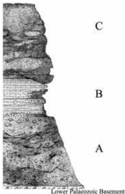
Figure 8 - Stratigraphic section
